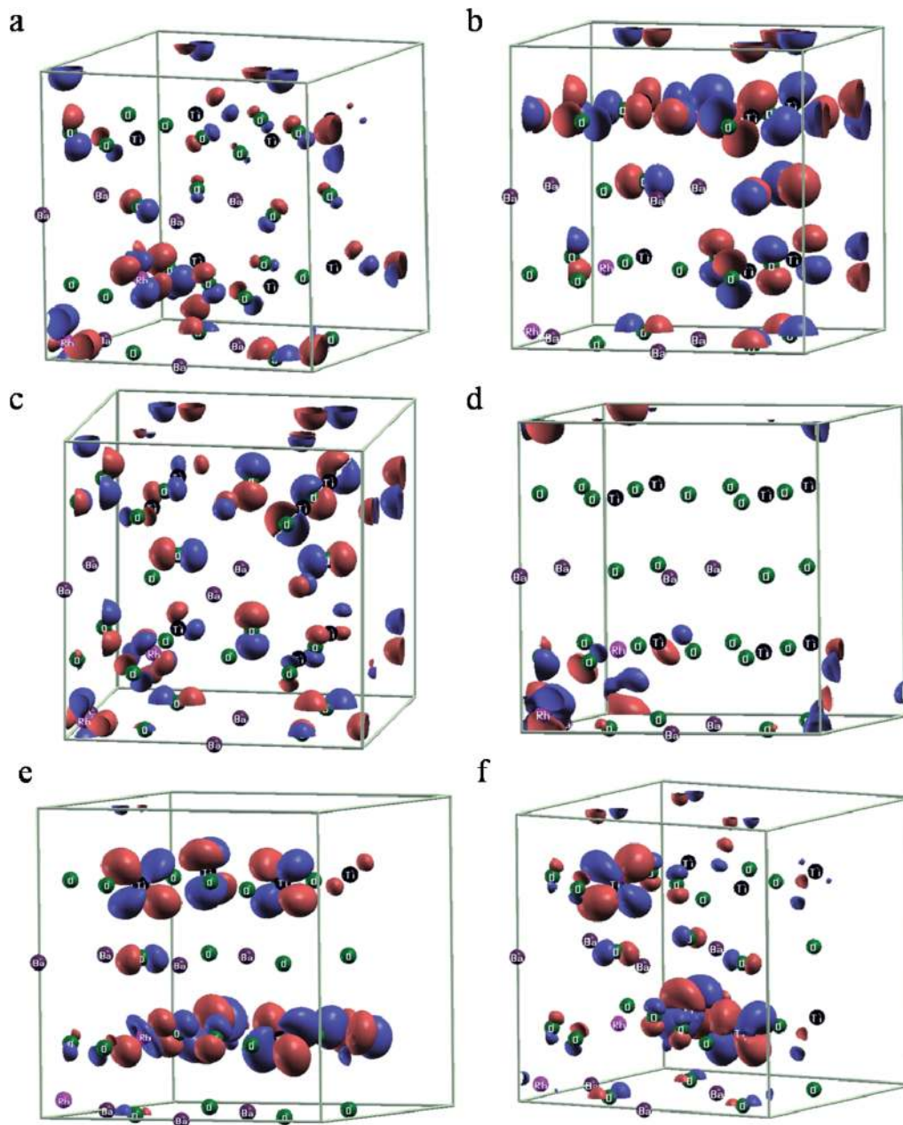
Fig. 3 Wavefunction visualization at the \Gamma point (a–f) corresponding to various energy levels I–VI in the pDOS in Fig. S1,† respectively, for case A. Red and blue colors indicate the positive and negative lobes of the orbitals.
