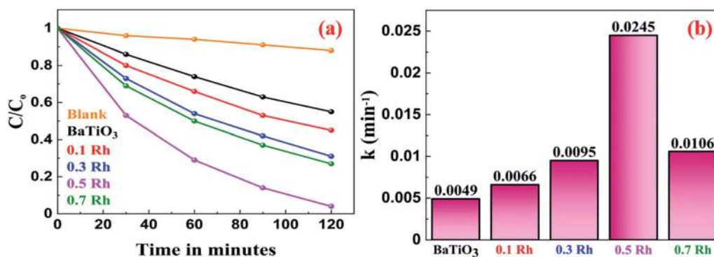
Fig. 11 (a) The photocatalytic degradation of MB and (b) the rate constants of the photocatalytic degradation of MB by the synthesized BaTiO 3 and Rh-doped BaTiO 3 .
