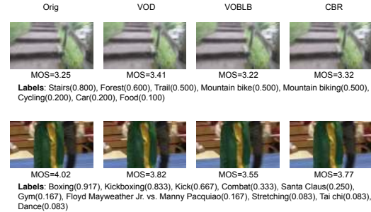
Figure 4. Low (top) & high (bottom) compression sensitivity
