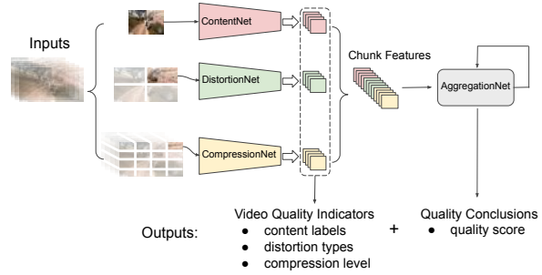
Figure 6. Overview of CoINVQ framework. Frames and chunks extracted from the input video are fed into three sub DNN models to extract corresponding features and quality indicators which are then aggregated to obtain the final quality score.
