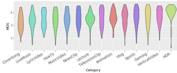
Figure 2. MOS distributions for original videos by content type.
