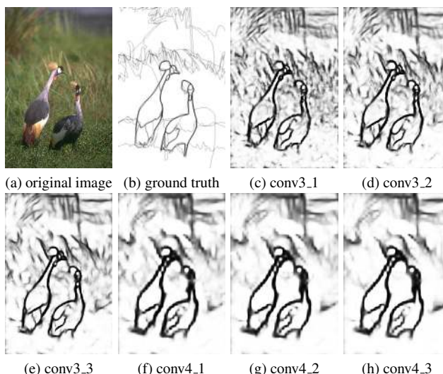
Figure 1: We build a simple network based on VGG16 [50] to produce side outputs of conv3_1 , conv3_2 , conv3_3 , conv4_1 , conv4_2 and conv4_3 . One can clearly see that convolutional features become coarser gradually, and the intermediate layers conv3_1 , conv3_2 , conv4_1 , and conv4_2 contain lots of useful fine details that do not appear in other layers.
