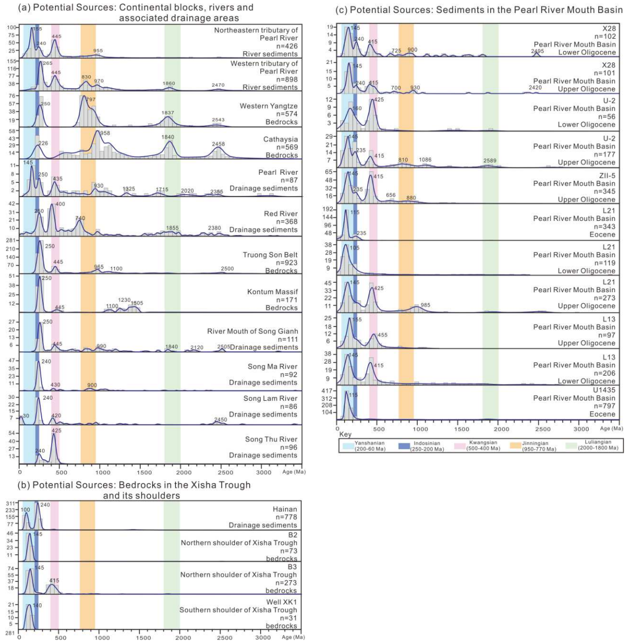
Figure 12 Kernel density estimate plots of analyzed U-Pb detrital zircon ages for potential sources of Oligocene sediment. See Supplementary Table S1 for all U-Pb age data acquired.
