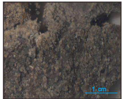
S3 (depth: 3297m; Lingshui Formation) gray fine sandstone
