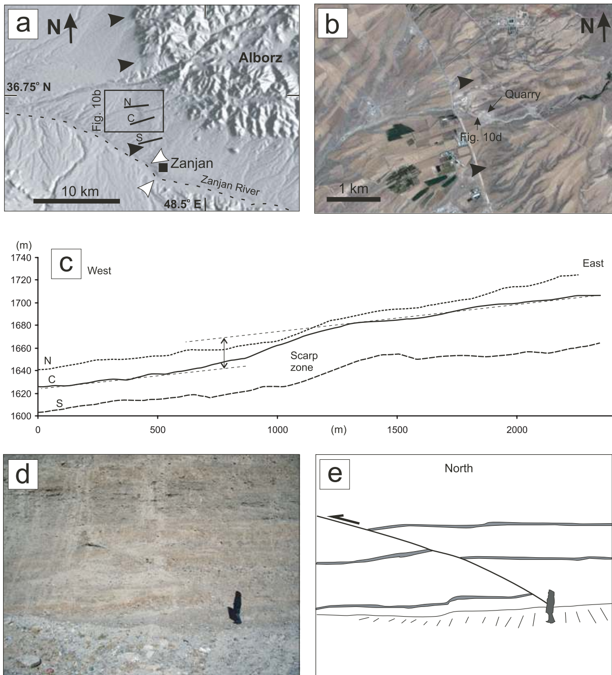
Figure 10. Quaternary faulting in the Zanjan region. (a) SRTM image of abrupt topographic fronts at the southwestern corner of the Alborz mountains. The NNW trending range front (black arrows) is interpreted as a right-lateral oblique-slip thrust, the North Zanjan Fault. White arrows show the right-lateral jog in the course of the Zanjan River. There are no magnitude >5 earthquakes in this region in either the instrumental or historical datasets. (b) Quickbird image (from Google Earth, ©2010 Google, ©2010 DigitalGlobe) of the topographic scarp (arrowed), interpreted as the location of the North Zanjan Fault. (c) Three topographic profiles (N,C,S) across the scarp highlighted in (b), including a reconstruction of the scarp height for the central profile. (d) Field photograph of a thrust in late Quaternary gravel, at the quarry highlighted in (b). (e) Interpretation of (d), highlighting reddish palaeosols developed within the gravels, offset by the thrust.
