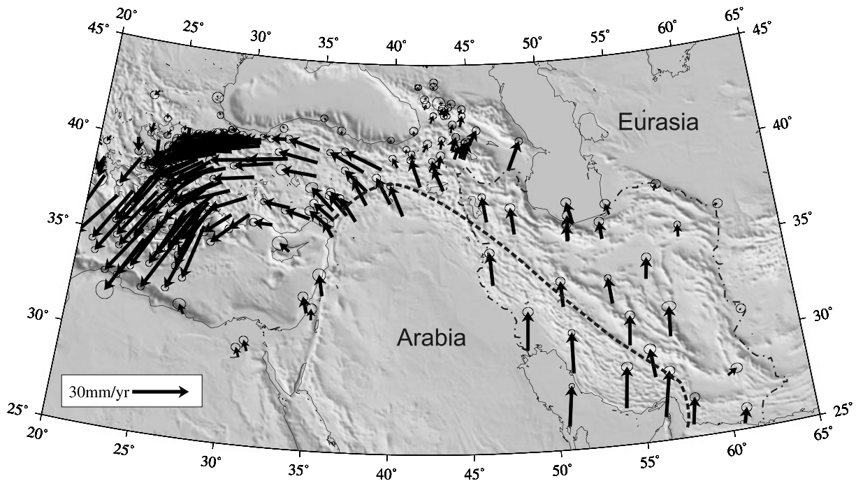
Figure 2. GPS-derived velocity field for the Arabia–Eurasia collision, with respect to a stable Eurasia reference frame (McClusky et al. 2000; Vernant et al. 2004). Thick dashed line shows approximate Arabia–Eurasia suture. Iran national border highlighted.
