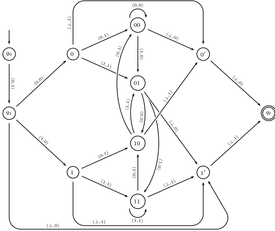
Figure 2: An example illustrating the proof of Lemma 9.
