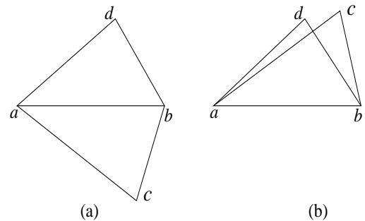
Fig. 1. Two first-order rigid formations with the same graph and the same distance values.
