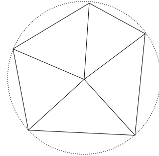
Fig. 3. Wheel graph W_6 .
