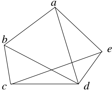
Fig. 2. A globally rigid formation in the plane.
