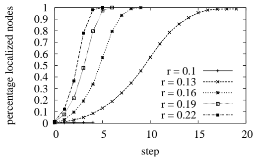
Fig. 8. Time-evolution of the number of localized nodes.
