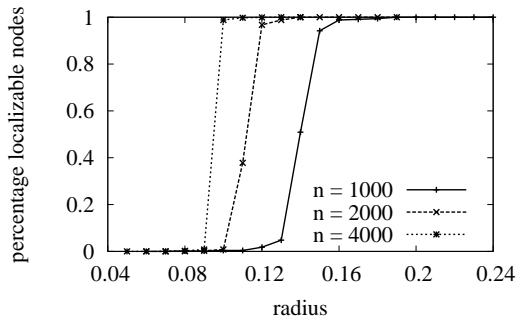
Fig. 6. Percentage of nodes localizable with 4-beacon ITP.
