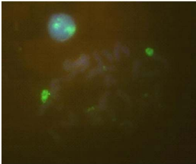
Figure 3. FISH image of metaphase using Whole Chromosome Staining probe (WCP) and chromosome 13 was seen as green signal
