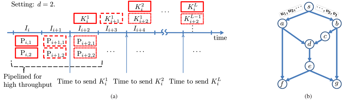
Fig. 1. a) This figure illustrates the packet and key disclosure schedule of source \mathcal{S} . In this example, network delay D is 0.9\delta and the key disclosure delay d is 2. \mathcal{S} sends two packets per interval. For the two packets P_{i,1} and P_{i,2} sent in interval I_i , \mathcal{S} releases the corresponding level j keys K_i^j in interval I_{i+dj} , by when P_{i,1} and P_{i,2} must have reached all level j nodes. Specifically, \mathcal{S} releases K_i^1, K_i^2, \dots, K_i^L for levels 1, 2, \dots , L in intervals I_{i+2}, I_{i+4}, \dots, I_{i+2L} respectively. For ease of understanding, we use the same box frame for packets sent in an interval and the corresponding level keys for that interval. b) \mathcal{S} sends multiple batches of messages \{u_i, v_i\}_i to nodes f and g over a skewed Butterfly network, where each link has unit capacity and unit delay. Node d buffers u_i and waits for v_i before transmitting u_i + v_i to node e . Due to pipelining, the achieved multicast throughput is still 2.
