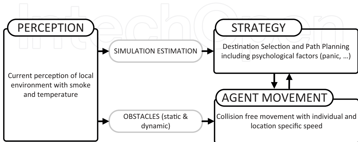
Figure 12. The high level description of the of the simulation algorithm proposed by Klugl et al. [13].
