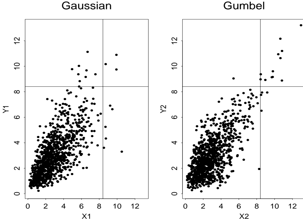
FIGURE 1. 1000 random variates from two distributions with identical Gamma(3,1) marginal distributions and identical correlation \rho = 0.7 , but different dependence structures.
