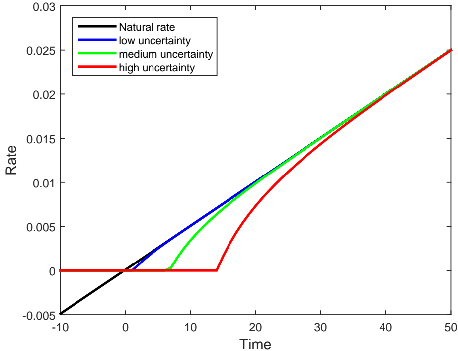
Figure 1: Optimal Lift-off in the Forward Looking Model
