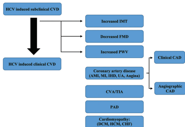
Fig. 1. Flowchart.
