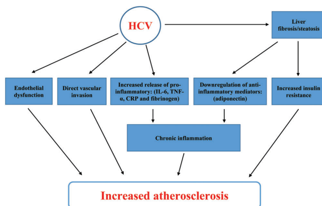
Fig. 2. Mechanism of HCV-induced CVD.
