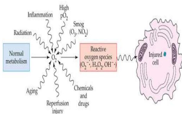
Figure 16. Formation of reactive oxygen species.
