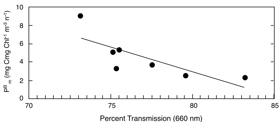
Figure 9. Maximal chlorophyll-normalized productivity ( P_m^B ) as a function of percent transmission (beam transmissometer; 660 nm) for stations inside the river plume during August 2005. Similar trends were obtained for other years. Photosynthesis irradiance curve data were obtained as described by Kudela et al. [2006].
