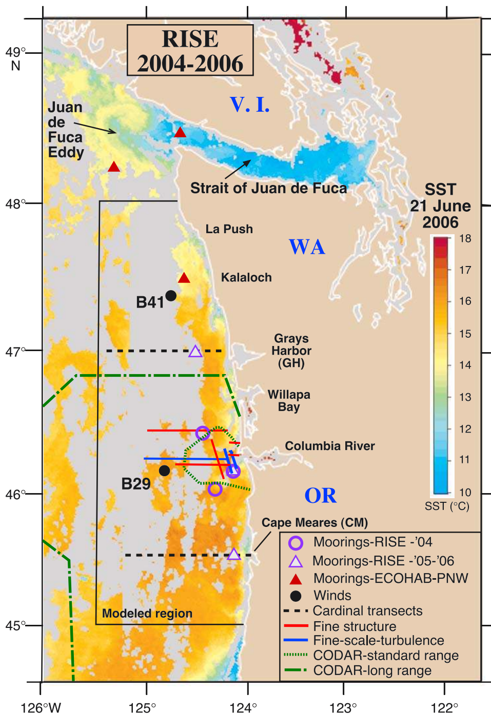
Figure 2. Locations of all sampling transects, moored sensor arrays and wind buoys, and CODAR ranges plotted on a satellite-derived sea surface temperature image on 21 June 2006. Regional physical features of interest are noted.
