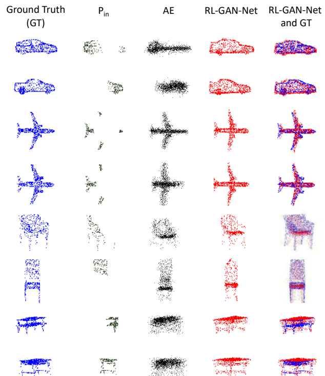
Figure 1: Qualitative results of point cloud shape completion given input data missing 70% of its original points. We present RL-GAN-Net , which observes a partial input point cloud data ( P_{in} ) and completes the shape within a matter of milliseconds. Even when input is severely distorted, our approach completes the shape with high-fidelity compared to the previous approach using autoencoder (AE) [1].
