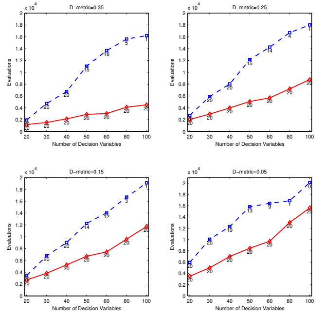
Fig. 23. The average number of function evaluations among the successful runs for reaching each of four given levels of D -metric v.s. the number of decision variables in two algorithms for F5. The marked number is the number of successful runs. The solid line is for RM-MEDA while dash line for GDE3.
