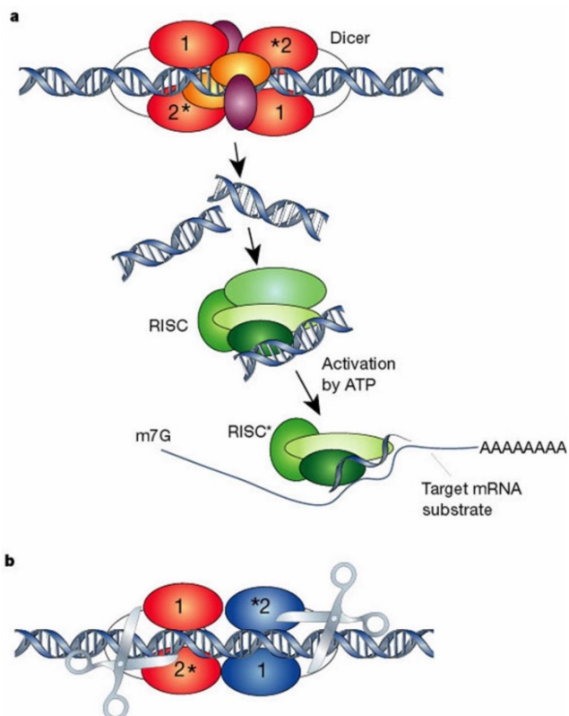
Figure 1. Model of Dicer and RNA-induced silencing complex (RISC) A. silencing initiate with enzyme Dicer and dsRNA is processed to convert the silencing trigger to ~22-nucleotide, small interfering RNAs (siRNAs), B. Dicer binding and cleaving dsRNA (*Cleavage into precisely sized fragments is determined by the fact that one of the active sites in each Dicer protein is defective. Different colors show two separate molecules of Dicer). Reprinted by permission from Macmillan Publishers Ltd: Nature, 418: 244-251, (2002)
