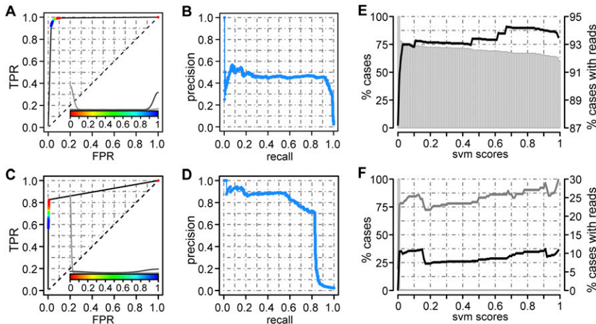
FIGURE 1. Evaluation of the classifier at 22°C. (A) Receiving Operating Characteristic (ROC) curve of the SVM classifier using scoring scheme score1 (see text). For each threshold of the score, the true positive rate (TPR) and false positive rate (FPR) values are represented in the x - and y -axes, respectively. The distribution of values for positive cases (dark gray) and negative cases (light gray) together with the color scale for the different thresholds used can be seen at the bottom of the graph. (B) Precision-recall curve of the SVM classifier using score1 . In the precision-recall curve, the TPR (recall) is represented in the x -axis, whereas the y -axis shows the precision, i.e., number of true positive cases for a given threshold over the total amount of cases predicted as positive. (C) ROC curve and (D) precision-recall curve for the SVM classifier using scoring scheme score2 (see text). (E,F) Cumulative distributions of predicted 3'ss that are validated by RNA-Seq reads obtained at 22°C, for annotated (E) and cryptic (F) 3'ss. The left y -axis represents the percentage of 3'ss that have a score2 higher than or equal to that given on the x -axis (gray bars). The right y -axis scale represents the percentage of cases with a score2 higher than or equal to that given on the x -axis and that can be validated using RNA-Seq reads that also validate the annotated 5'ss (black line) or that may validate other 5'ss (gray line).
