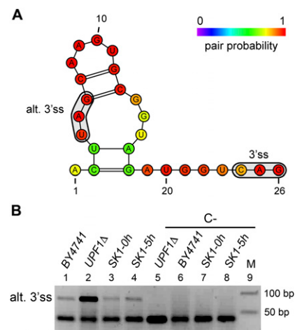
FIGURE 2. Experimental validation of a predicted alternative 3' ss in VPS75 . (A) Predicted optimal secondary structure between the BS and the annotated 3' ss for the VPS75 gene, discarding the 8 nt after the BS. The 3' ss and the alternative 3' ss (alt. 3' ss) tested are boxed in the picture. The color of the nucleotides represents the pair probability of the bases in the optimal secondary structure. For nucleotides outside the secondary structure, the color represents the accessibility of the nucleotide (one-pair probability) in the same scale. (B) RT-PCR validation of the alternative 3' ss of the VPS75 gene using specific primers in different yeast strains and conditions. Lanes 1–4 show the RT-PCR product of the alternative 3' ss using RNA from strains BY4741 (lane 1), UPF1 Δ (lane 2), and SK1 at time zero of meiosis (lane 3) and after 5 h (lane 4) (Materials and Methods). Lanes 5–8 show the corresponding negative controls without AMV reverse transcriptase. Lane 9 contains the markers, with the corresponding lengths indicated on the right. Bands corresponding to the alternative and annotated 3' ss are indicated. The band for the alternative 3' ss appears in all the conditions tested, although it is more highly expressed in UPF1 Δ.
