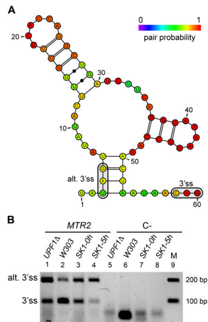
FIGURE 3. Experimental validation of a predicted alternative 3'ss in the 5' UTR in MTR2 . (A) Predicted optimal secondary structure between the BS and the annotated 3'ss, discarding the first 8 nt after the BS A, in the 5' UTR of the MTR2 gene. The 3'ss and the alternative 3'ss (alt. 3'ss) tested are boxed in the picture. The color of the nucleotides represents the pair probability of the bases in the optimal secondary structure. For nucleotides outside the secondary structure, the color represents the accessibility of the nucleotide (one-pair probability) in the same scale. (B) RT-PCR validation of the splicing pattern of the MTR2 gene in different yeast strains. Lanes 1–4 show analyses of MTR2 using RNA from strains UPF1Δ (lane 1), W303 (lane 2), and SK1 at time zero of meiosis (lane 3) and after 5 h (lane 4) (Materials and Methods). Lanes 5–8 show the corresponding negative controls without AMV reverse transcriptase. Lane 9 contains the markers, with the corresponding lengths indicated on the right. Bands corresponding to the alternative and annotated 3'ss are indicated. The band for the alternative 3'ss appears in the strains UPF1Δ and W303 and during meiosis ( SK1-0 h and SK1-5 h ).
