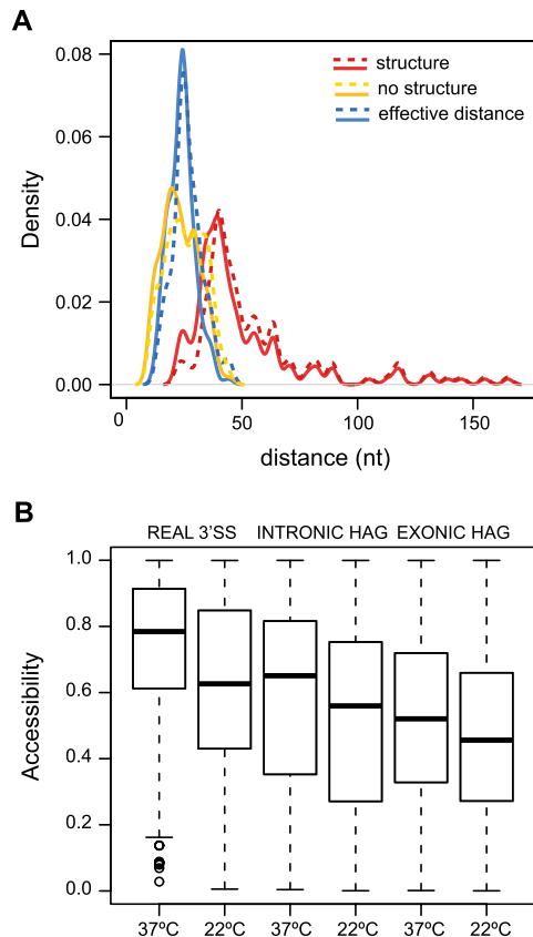
FIGURE 4. Effective distance and accessibility properties of 3' splice sites. (A) Comparison of BS-3'ss length distribution at 22°C (continuous) and 37°C (dashed lines). The plot shows the length distribution of BS-3'ss regions with a secondary structure (red) and for those without a predicted secondary structure (yellow). In the cases in which a secondary structure is predicted, the distribution of the effective distances is also shown (blue). (B) Box plots representing the accessibility distributions at 22°C and 37°C for real 3'ss, intronic HAGs, and exonic HAGs. Accessibility values are shown on the y -axis, which can vary between 0 (always covered by a secondary structure) and 1 (never covered by a secondary structure).
