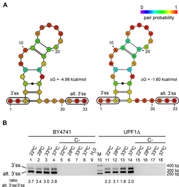
FIGURE 5. Experimental validation of an alternative 3'ss modulated by temperature in YLR211C . (A) Predicted optimal secondary structure between the BS and the alternative 3'ss predicted at 22°C (left) and at 37°C (right) for the YLR211C gene, discarding the first 7 nt after the BS. The 3'ss and the alternative 3'ss tested (alt. 3'ss) are boxed in the picture. The color of the nucleotides represents the pair probability of the bases in the secondary structure. For nucleotides outside the secondary structure, the color represents the accessibility of the nucleotide (one-pair probability) in the same scale. Even though the optimal secondary structure does not change, the stability of the optimal secondary structure decreases with temperature ( \Delta G 22°C = -4.98 kcal/mol; \Delta G 37°C = -1.60 kcal/mol). Furthermore, a difference in the accessibility of the nucleotides from the alternative 3'ss can be observed, as calculated in Materials and Methods (see text) or as calculated from the optimal structure (average accessibility at 22°C, 0.948; accessibility at 37°C, 0.973). (B) RT-PCR validation of the splicing pattern in the YLR211C gene in two different yeast strains and at different temperature conditions. Cells were grown at the specified temperature for at least three duplications. The picture shows the RT-PCR analyses of YLR211C using RNA from strains BY4741 (lanes 1–9) and UPF1Δ (lanes 11–18). Lanes labeled with C- correspond to the negative controls with no AMV reverse transcriptase. Lane 10 contains the markers, with the corresponding lengths indicated on the right. Below, we include the rate per lane of the proportions of mRNA for the predicted alternative 3'ss over the annotated 3'ss.
