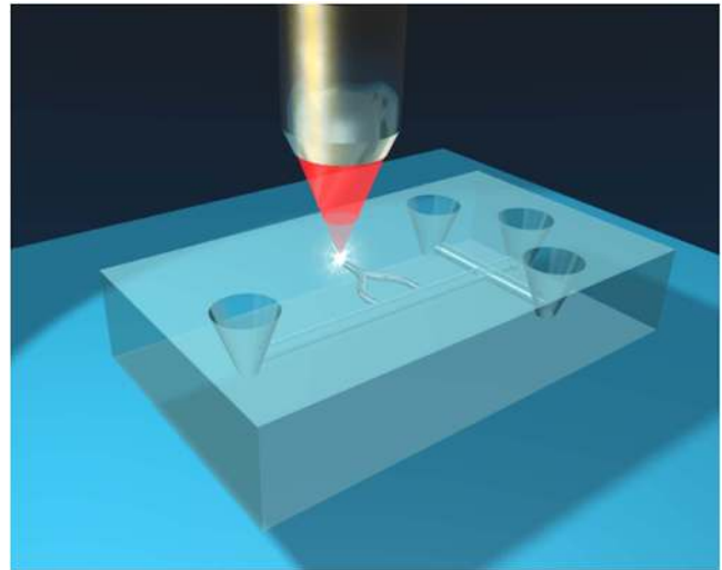
Figure 1. FLM can create optofluidic devices, encompassing optical waveguides and microfluidic channels, directly buried inside a glass sample.
