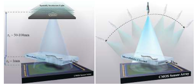
Figure 7. Left: schematic setup of holographic optofluidic microscopy (HOM). Reproduced from [74]. CC BY 3.0. Right: schematic setup of holographic optofluidic tomography (HOT). Reprinted from [83], with the permission of AIP Publishing.
