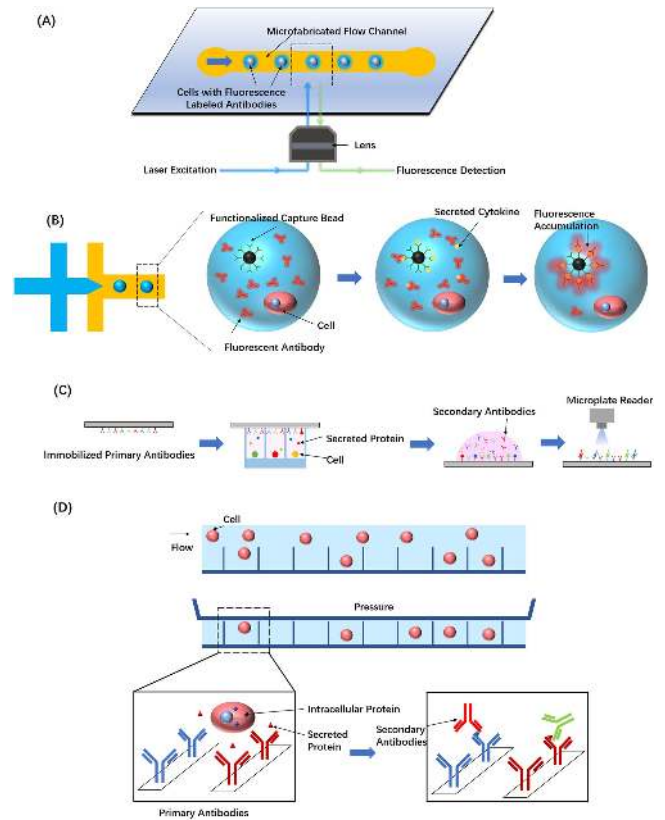
Figure 23. Key developments of optofluidic systems enabling high-throughput single-cell protein characterization, which includes (a) optofluidic fluorescent flow cytometry; (b) droplet-based optofluidic flow cytometry; (c) large-array microwells (microengraving); and (d) large-array microchambers (barcode microchips).
