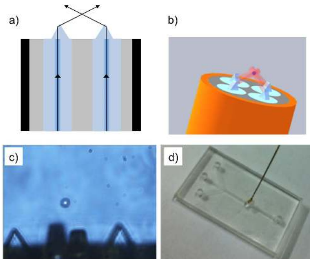
Figure 19. (a) Cross section of the FOT probe presented in [140]: beams propagating in two symmetrically positioned fibers are reflected at the interface between microprisms and the outer medium; (b) isometric view of the FOTs; (c) red blood cell trapped by the FOTs in hypotonic solution; (d) picture of a microfluidic chip where the FOTs have been inserted. Adapted by permission from Macmillan Publishers Ltd: Scientific Reports [140], Copyright 2013.
