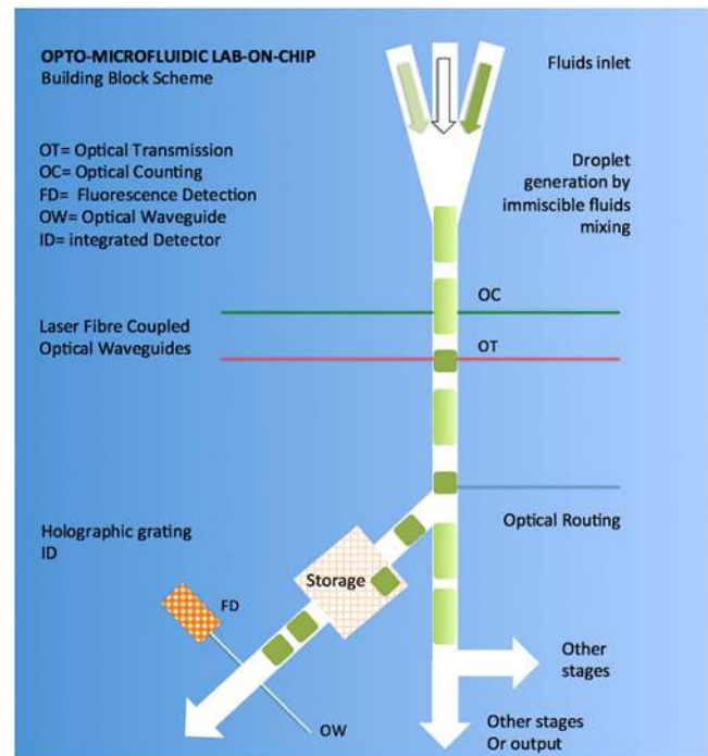
Figure 4. LiNbO 3 -based optofluidic platform.
