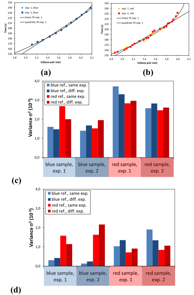
Figure 25. Migration time (linear scale) versus base-pair size (logarithmic scale) of (a) 12 blue-labeled and (b) 23 red-labeled DNA molecules simultaneously migrated and separated in experiment 1 (circles) and experiment 2 (squares). Linear and quadratic fits (solid lines) shown only for experiment 1. Variance \sigma^2 measured in experiment 1 or 2 from (c) the linear fit and (d) the quadratic fit, obtained from the measured reference data from the same or the different experiment. Reproduced from [182]. CC BY 3.0.
