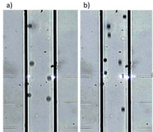
Figure 20. Microfluidic all-glass device with a liquid channel of a rectangular cross section; the channel is 100 \mu\text{m} wide. Details may be found in [152]. Shown are images of 5 \mu\text{m} diameter polystyrene beads in water, visualized by standard bright-field microscopy. Laser-written waveguides in the glass chip were in the focal plane; bright spots indicate scattered laser light coupled into two opposing waveguides. (a) Acoustic vertical focusing turned off. (b) Acoustic vertical focusing turned on. Scattering by trapping laser light on the beads illustrates nicely the acoustic prefocusing of the beads to the plane of the waveguides. [152] © Springer-Verlag Berlin Heidelberg 2015. With permission of Springer.
