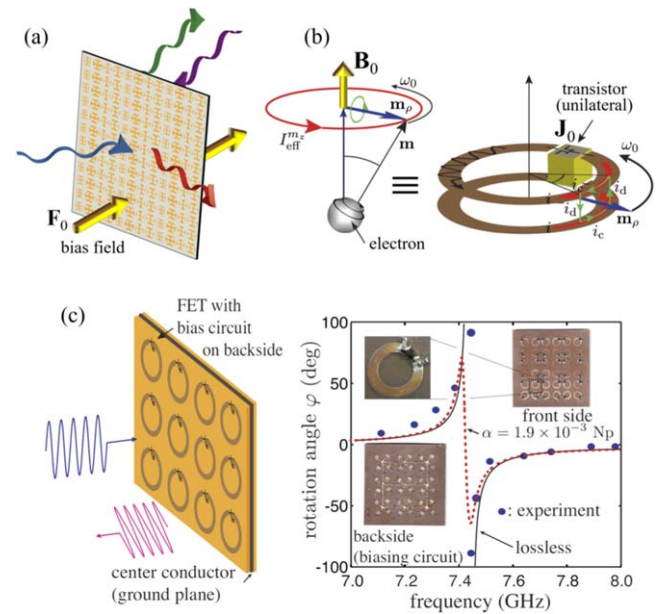
Figure 12. (a) Generic representation of a nonreciprocal metasurface, with bias field \mathbf{F}_0 . (b) Magnetless transistor-loaded ring metamaterial particle, mimicking electron spin precession in ferrites, with current \mathbf{J}_0 operating as the biasing field [110–112]. (c) Reflective Faraday ring metasurface based on the particle in (b). (Left) Perspective view of the metasurface structure. (Right) Faraday rotation angle versus frequency obtained theoretically from the equivalent magnetic Polder tensor (dashed and solid curves) and experimentally from the prototype shown in the insets (dots) [110].
