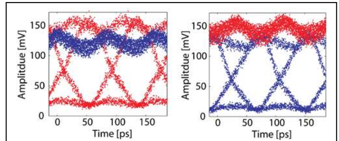
Figure 2 – Simultaneous cloaking and data transmission for wavelength-multiplexed channels. Cloaking along the short-wavelength (blue) channel (left) or along the long-wavelength (red) channel (right). Reproduced with permission of OSA from [6].
