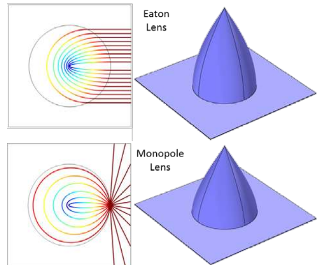
Figure 1 – Ray tracing in graded index profiles and the equivalent homogeneous surfaces for the Eaton lens and a Monopole lens.
