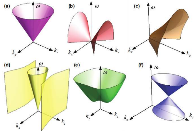
Figure 1 – Conceptual illustration of the nonlocal TO extension in the frequency ( \omega )-wavevector ( \mathbf{k}_x, \mathbf{k}_z ) phase space (see [3]). (a) Conical dispersion surface of a homogeneous medium. (b) Hyperbolic dispersion (purely imaginary transformation component). (c) One-way, nonreciprocal propagation (non-centersymmetric transformation). (c) Additional extraordinary wave (multivalued transformation). (d) Frozen mode (stationary inflection point). (f) Dirac-point conical singularity (phase-space shift).
