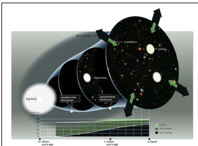
Figure 2. Expansion of the universe. The observed expansion is dominated by unobserved dark energy (black) and dark matter (olive green). Both represent a mystery, in particular dark energy, that appears to generate repulsive gravity. Figure reproduced from https://www.nobelprize.org/ popular material to the 2011 Nobel Prize in physics.
