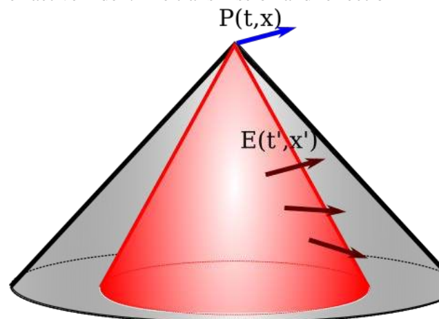
Figure 2: The support (red) of the intergral kernel associated with a temporally and spatially dispersive medium, inside the backward lightcone (grey). The Polarisation P(\mathbf{t}, \mathbf{x}) depends on the electric field E(\mathbf{t}', \mathbf{x}') in its past lightcone.
