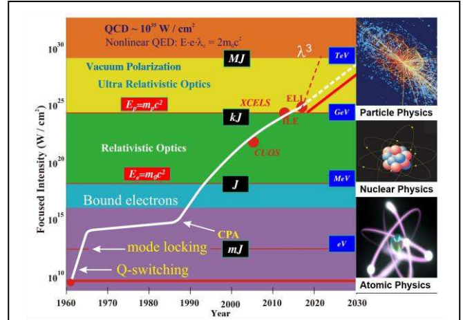
Figure 1 – Laser Intensity through the years. The dashed line corresponds to what could be obtained with significant increases in beam size or by increasing the number of beams. The red-dashed line corresponds to the “short cut” obtained through compression technique to sub-attosecond pulse durations. The plot has evolved from an early version first presented in [4].
