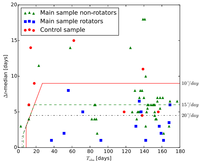
Figure 1. Season length and median cadence for the first season data. Broken lines limit areas where rotations at rates of 10, 15 and 20 \text{deg d}^{-1} can be detected (see Section 3.3 for details). Only objects with \Delta t -median \leq 20 were left for the more detailed view.
