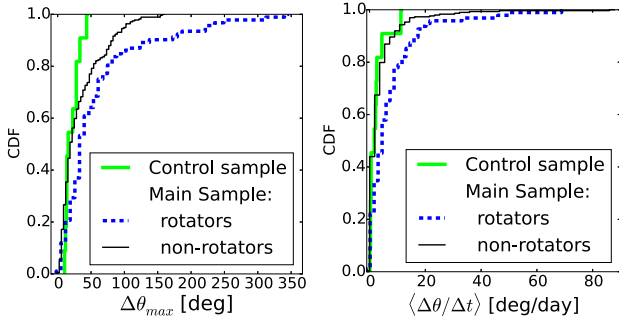
Figure 4. CDFs of \Delta\theta_{\max} and average rates for the main sample rotators (95 EVPA swings), the main sample non-rotators (298 swings) and control sample sources (11 swings). See Section 3.4 for details.
