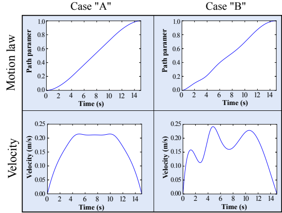
Figure 5: Given motion laws and computed end-effector velocities.
