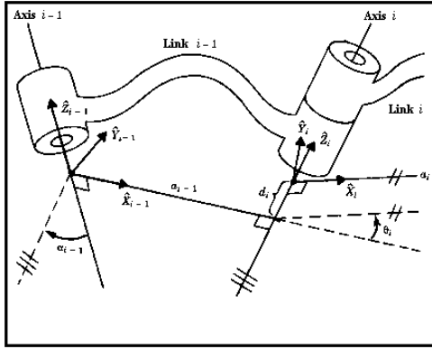
Fig. 3. Link Transformations
