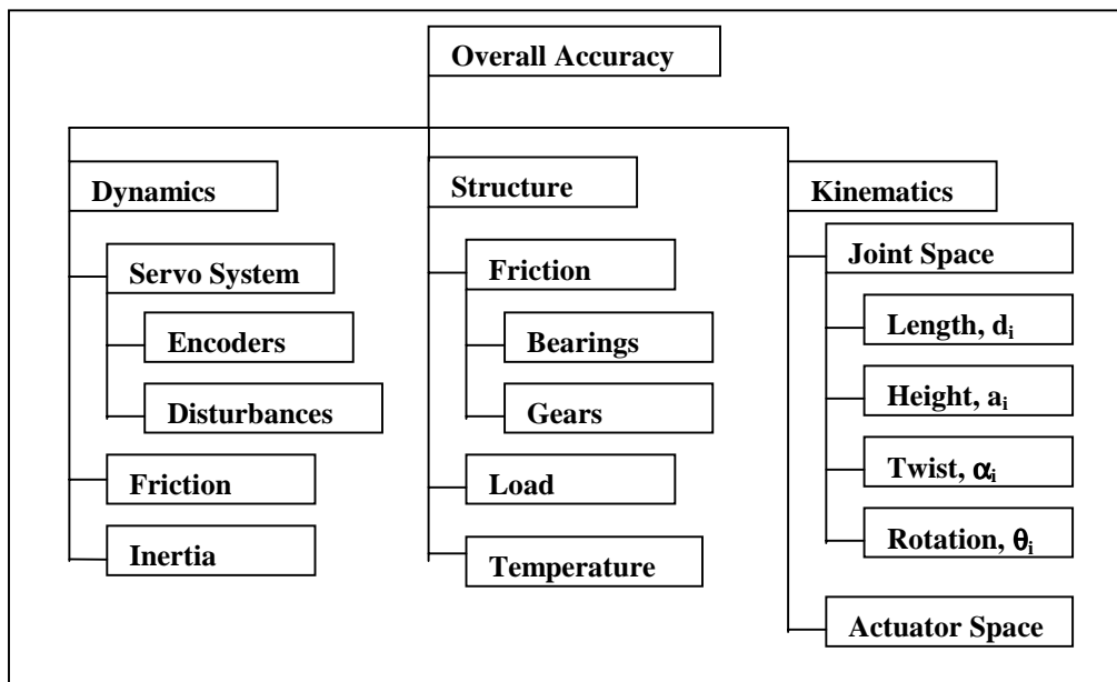
Fig. 4. Error Tree.
