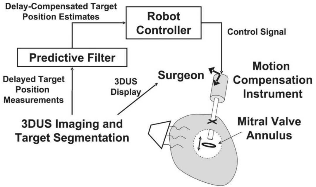
Fig. 1. Motion compensation system. Time-delayed position measurements of the target are provided to a filter which uses prediction to compensate for delay. These are fed-forward to the controller of the one-DOF MCI to synchronize with the target motion. The surgeon holds the instrument and navigates its end-effector to the target using 3DUS imaging.
