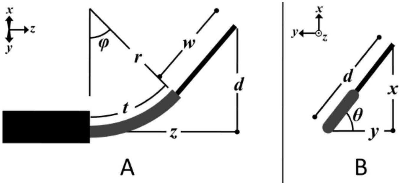
Fig. 9. Lateral planar view (A) and axial proximal-to-distal view (B) of concentric tube and cauterizing wire extending from the endoscope tip.
