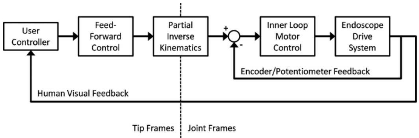
Fig. 10. Robotic endoscope control system schematic.
