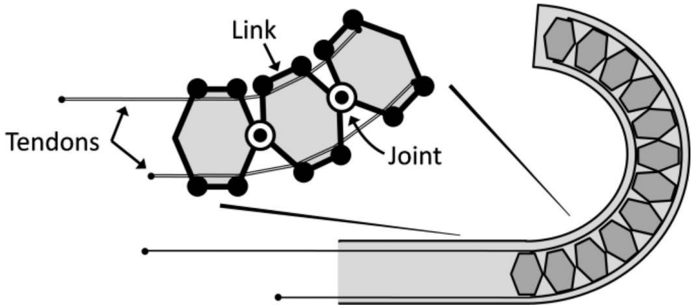
Fig. 2. Two-dimensional mechanical design for an endoscope tip.
