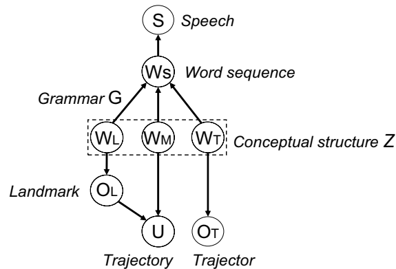
Figure 7. Graphical model of lexicon and grammar
