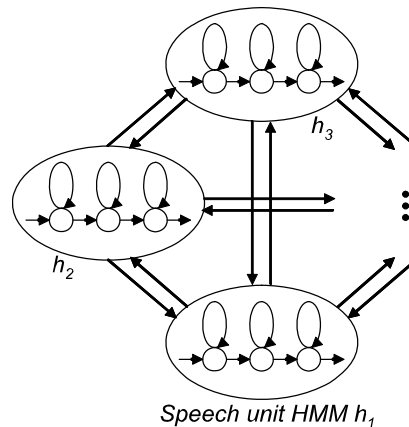
Figure 3. Structure of HMM for learning speech units
