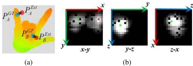
Figure 2: (a) Illustration of joint estimation in single view. Blue points are true locations, and red points are estimated locations. The little finger tip is misestimated on the background and the middle finger tip is misestimated on the hand palm. (b) Illustration of ambiguous estimation. Despite the heat-map of x - y view contains two hotspots which are hard to choose, from the heat-map of z - x view, it is easy to find that the x value is small with high confidence. Thus, the left hotspot in x - y view’s heat-map is true.
