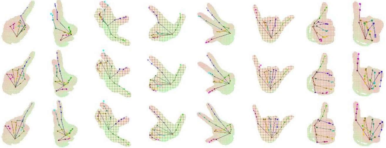
Figure 9: Qualitative results for dataset in [21] of three approaches: single view regression (in the first line), our multi-view regression with coarse fusion (in the second line) and our multi-view regression with fine fusion (in the third line). We show the estimated hand joint locations on the depth image. Different hand joints and bones are visualized using different colors. This image is best viewed in color.
