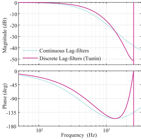
Fig. 7: Frequency response of the continuous lag-filters and the discrete lag-filters using the Tustin rule with pre-warping at the resonance frequency.
