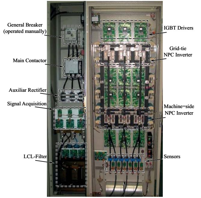
Fig. 11: 100 kVA Experimental set-up.
