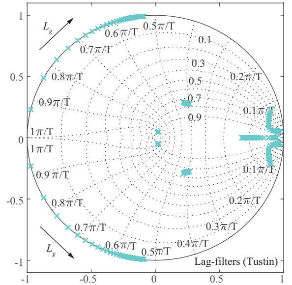
Fig. 9: root locus in the z -plane when varying L_g from 80% to 1000% (from 0.2 mH to 2.5 mH) for the lag-filter using the Tustin rule with pre-warping.
