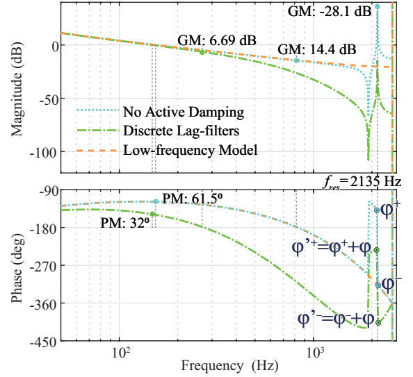
Fig. 8: Bode plot for the open-loop transfer function with no lag-filters (no active damping procedure) and the lag-filters for active damping. The figure also shows the open-loop transfer function for the low-frequency model.
