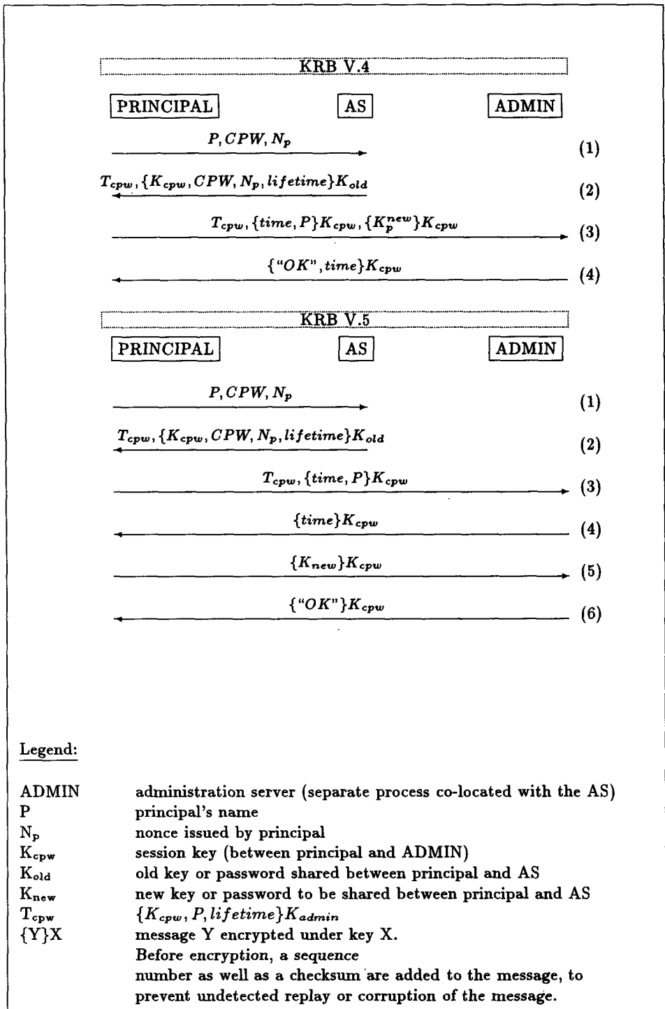
Fig. 1. The Kerberos CPW protocols
