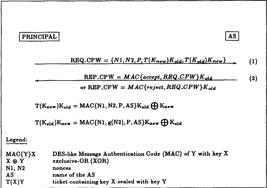
Fig. 2. Secure and fault-tolerant CPW protocol
