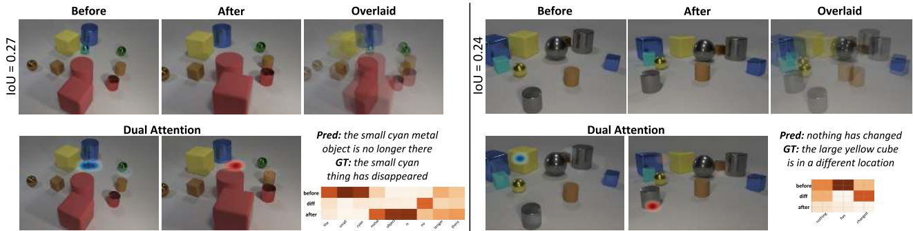
Figure 6: Qualitative examples of DUDA. The left is an example in which DUDA successfully localizes the change and generates correct descriptions with proper modulations among “before”, “diff”, and “after” visual features. The right example is a failure case. We observe that significant viewpoint shift leads to incorrect localization of the change, thus confusing the dynamic speaker.
