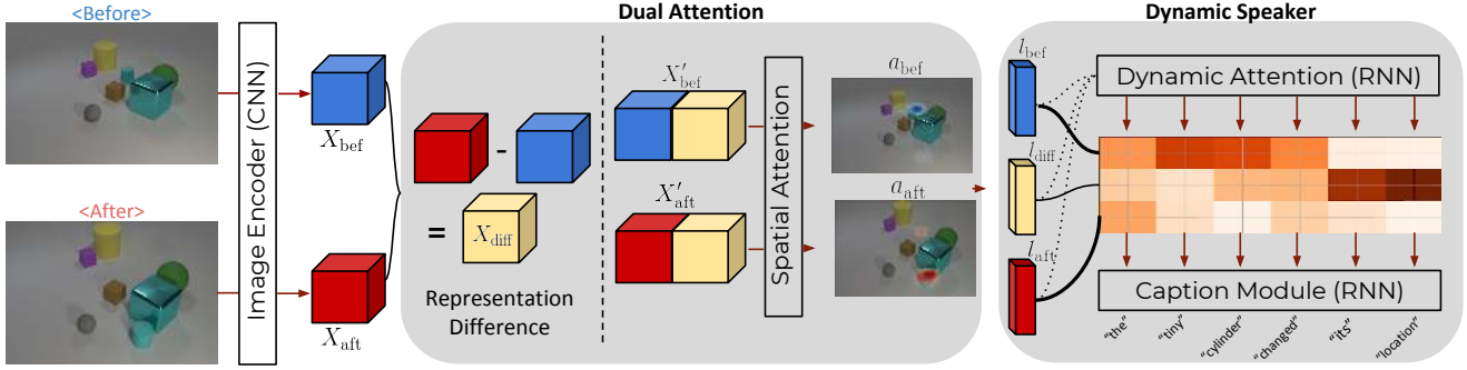
Figure 2: Our Dual Dynamic Attention Model (DUDA) consists of two main components: Dual Attention (subsection 3.1) and Dynamic Speaker (subsection 3.2).
