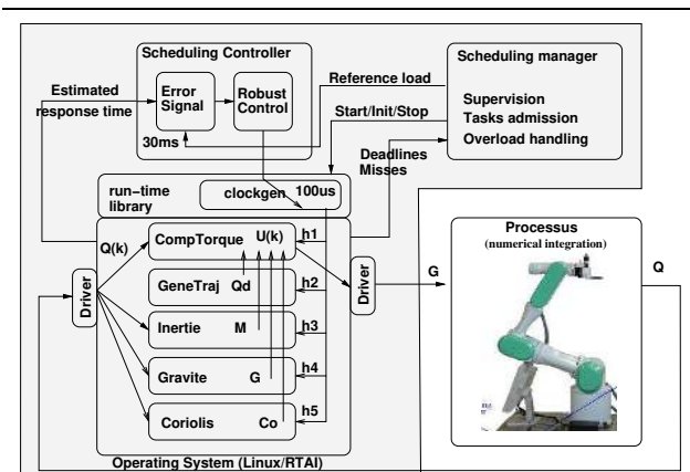
Figure 8. Feed-back scheduling experiment
