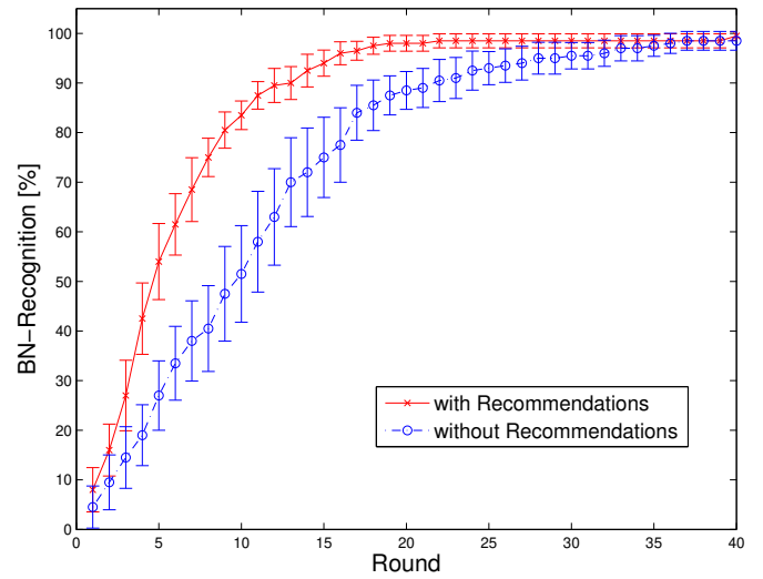
Figure 5: Convergence comparison of scheme with and without recommendations in respect to BN-recognition.
