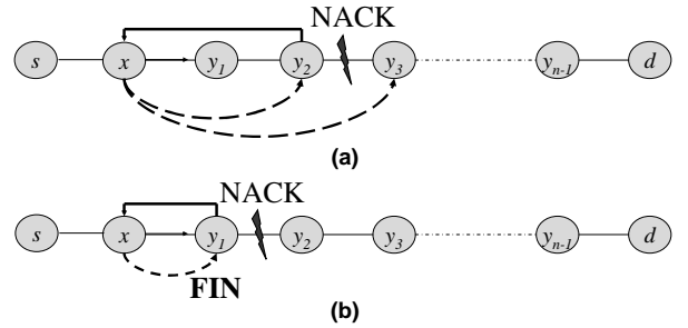
Figure 1: Processing of NACKs.
