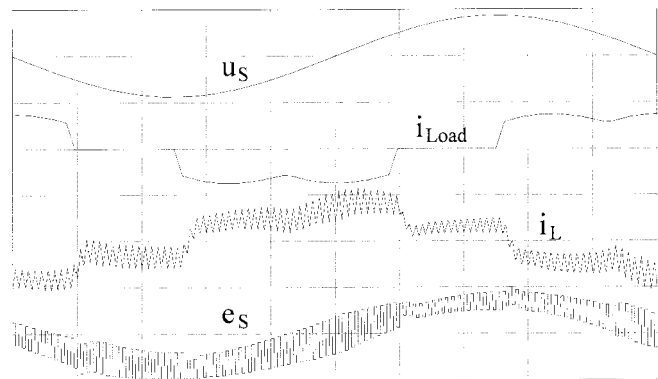
Fig. 8. Simulated active filter behavior with the classical estimation technique: u_s (80 V/div), i_{Load} (12 A/div), i_L (12 A/div), e_s (150 V/div), time scale (2 ms/div).
