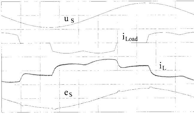
Fig. 9. Simulated active filter behavior with a bandpass filter in the estimation algorithm: u_s (80 V/div), i_{Load} (12 A/div), i_L (12 A/div), e_s (150 V/div), time-scale (2 ms/div).
