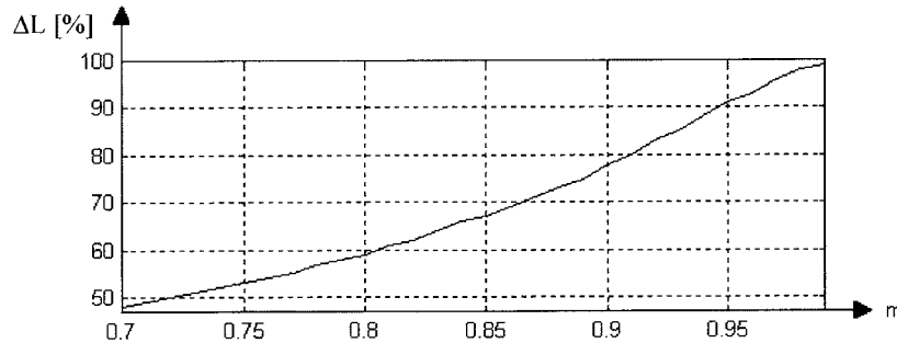
Fig. 7. Relationship between the stability margin \Delta L\% and the magnitude of the bandpass filter poles m .
