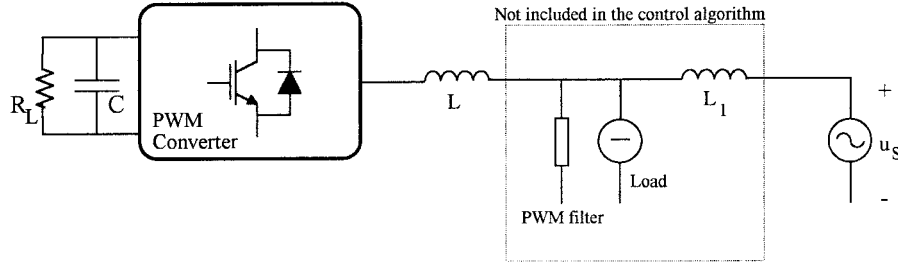
Fig. 3. Simplified representation of Fig. 1.
