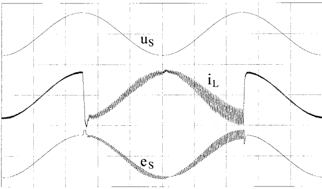
Fig. 10. Simulated PWM rectifier behavior with the classical estimation technique: u_s (100 V/div), i_L (12 A/div), e_s (150 V/div), time-scale (4 ms/div).
