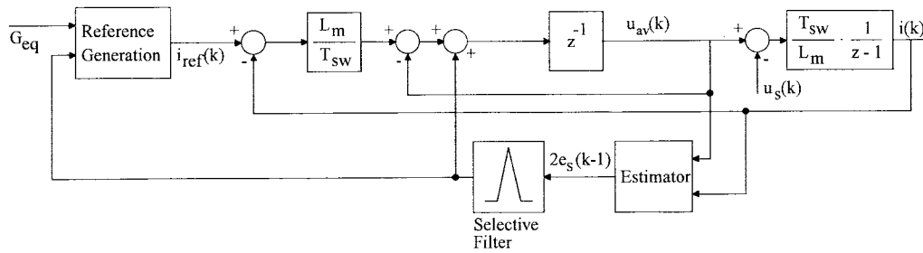
Fig. 6. Block diagram of the proposed control solution.
