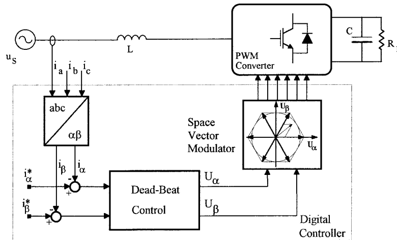
Fig. 2. Basic scheme of the digital dead-beat current regulator.
