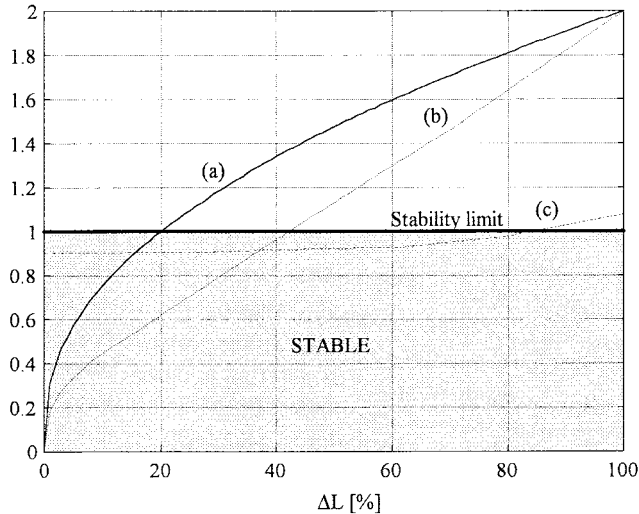
Fig. 4. Absolute value of the maximum closed-loop plant eigenvalue as a function of the relative estimation error on L . Solid line (a): line voltage conventional estimation; dashed line (b): reference calculation based on voltage estimation; dash-dotted line (c): proposed estimation technique.
