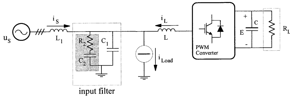
Fig. 1. Basic scheme of the system with the PWM converter.
