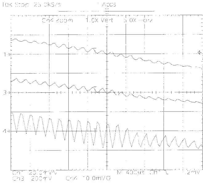
Fig. 14. Test condition: no filter on the estimated line voltage; V_{dc} = 120 V; \Delta L\% = 12\% ; time scale: 400 \mu s/div; rectifier mode. Upper trace: estimated line voltage (200 mV/div). Middle trace: line-to-neutral measured voltage (40 V/div). Lower trace: phase current (1 A/div).
