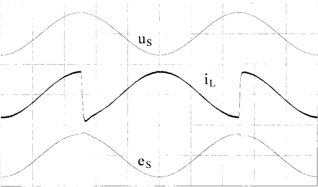
Fig. 11. Simulated PWM rectifier behavior with a bandpass filter in the estimation algorithm: u_s (100 V/div), i_L (12 A/div), e_s (150 V/div), time-scale (4 ms/div).
