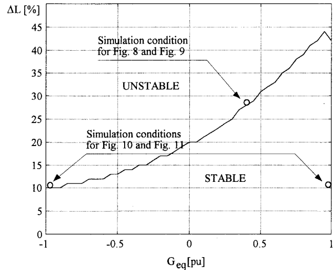
Fig. 5. Absolute value of the maximum relative error on the converter inductance L as a function of the G_{\text{eqpu}} . The simulated conditions, which give the results reported in Section V, are explicitly indicated.
