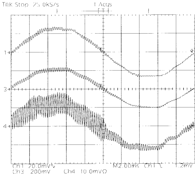
Fig. 13. Test conditions: no filter on the estimated line voltage; V_{dc} = 120 V; \Delta L\% = 12\% ; time-scale: 2 ms/div; rectifier mode. Upper trace: estimated line voltage (200 mV/div). Middle trace: line-to-neutral measured voltage (40 V/div). Lower trace: phase current (1 A/div).
