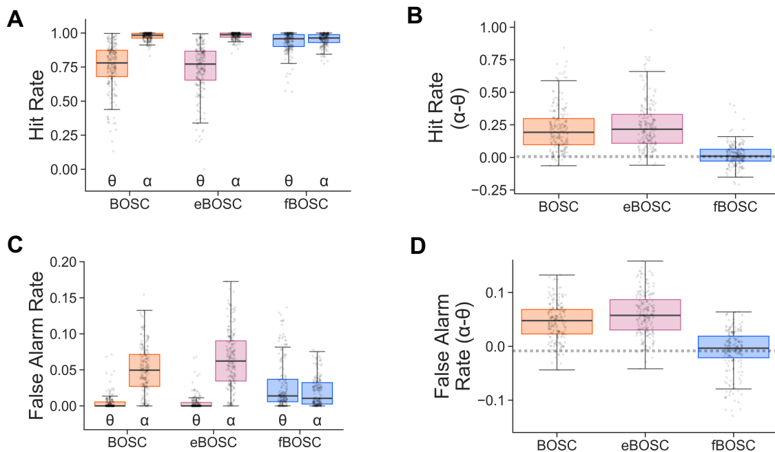
FIGURE 4 Simulations were performed using data with a non-linear 1/f power spectrum and embedded theta or alpha bursts (SNR = 5). BOSC, eBOSC and fBOSC were used to detect these oscillatory bursts. The (A) hit rate and (C) false alarm rate of theta and alpha burst detection are plotted for all three methods. The difference in (B) hit rate and (D) false alarm rate between theta and alpha burst detection is also plotted, with an additional dotted line at 0. Across all plots, individual data points correspond to each simulated trial.
