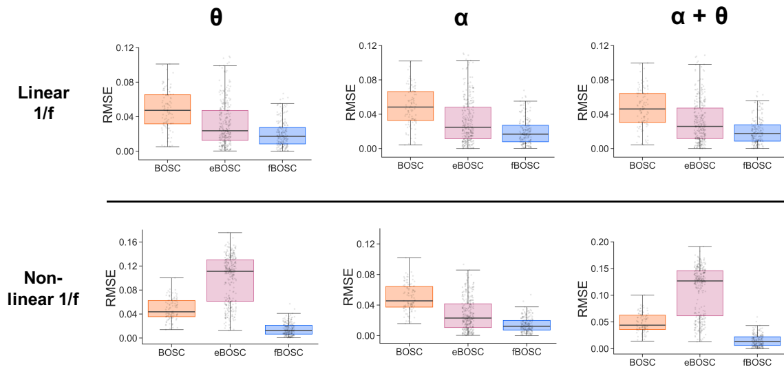
FIGURE 2 Simulations were performed using data with either a linear or non-linear background 1/f power spectrum. These data were then combined with simulated bursts in the theta-band alone (4 Hz), alpha-band alone (10 Hz), or both the theta and alpha-bands (4 Hz and 10 Hz). The SNR of the bursts was set at 5. For each set of simulations, the root mean squared error (RMSE) between the estimated and actual 1/f fit was plotted for BOSC, eBOSC and fBOSC. Individual data points correspond to RMSE values from each simulated trial.
