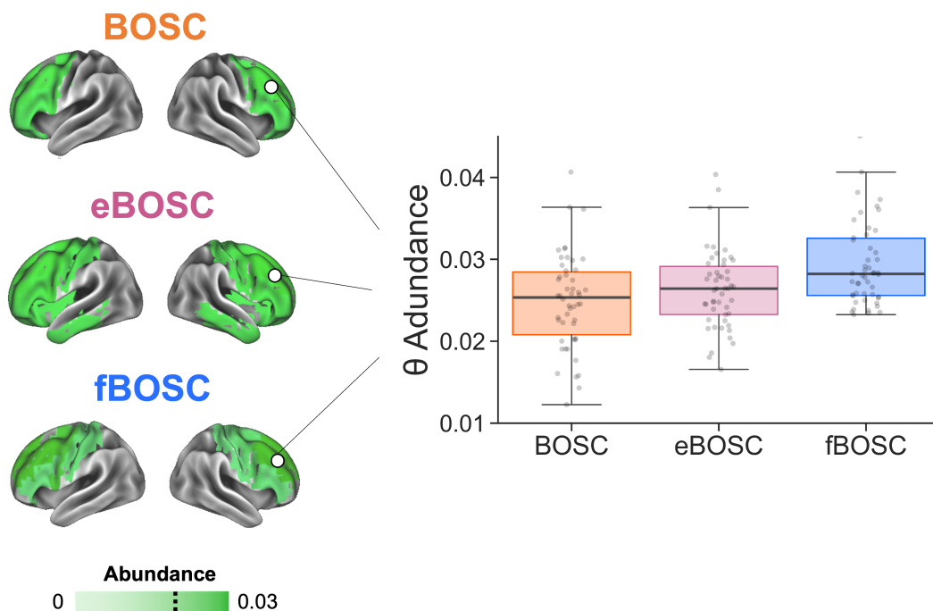
FIGURE 6 Using resting state MEG data, theta (3-7 Hz) burst abundance was quantified as the duration of rhythmic episodes relative to the length of the recording. The abundance values were plotted on a whole brain mesh separately for BOSC, eBOSC and fBOSC, thresholded at p < 0.02 for illustrative purposes. Abundance values from the right frontal cortex are plotted on the right panel separately for each method, with individual data points corresponding to each participant.
