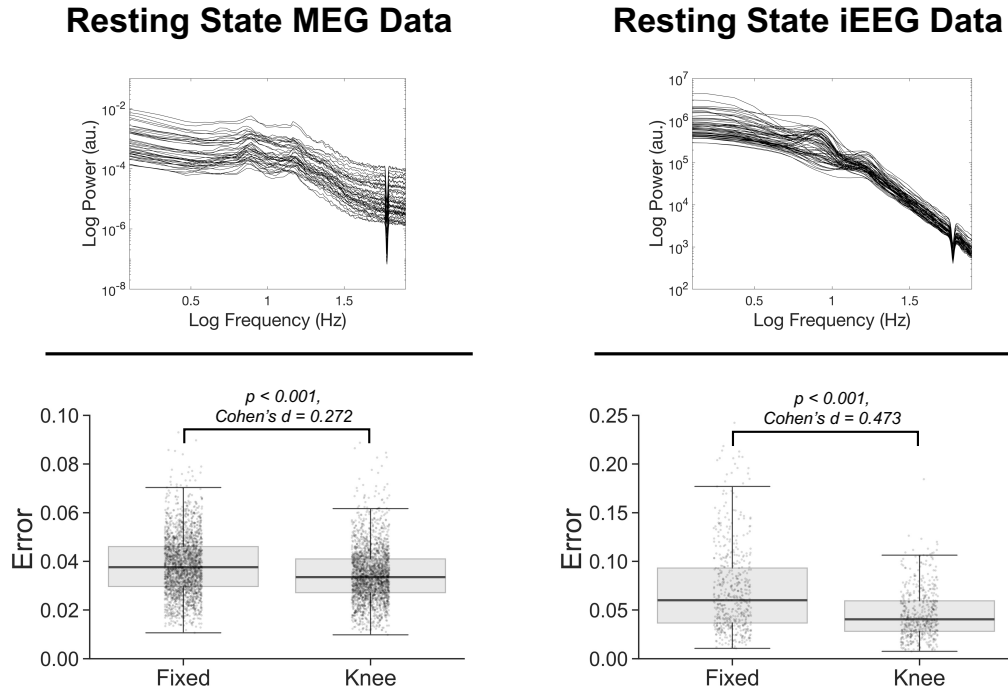
FIGURE 5 Neural power spectra are often non-linear. The top panels show power spectra plotted on a log scale from one example MEG dataset and one iEEG dataset. Individual lines correspond to ROIs (MEG) or electrodes (iEEG). Note the prominent knee in the power spectrum below \sim 8 Hz. The bottom panel shows the error when modelling the 1/f power spectrum as linear (fixed) or non-linear (can contain a knee parameter), using FOOOF (Donoghue et al., 2020b). Individual data points correspond to ROIs across participants (MEG) or electrodes across patients (iEEG).
