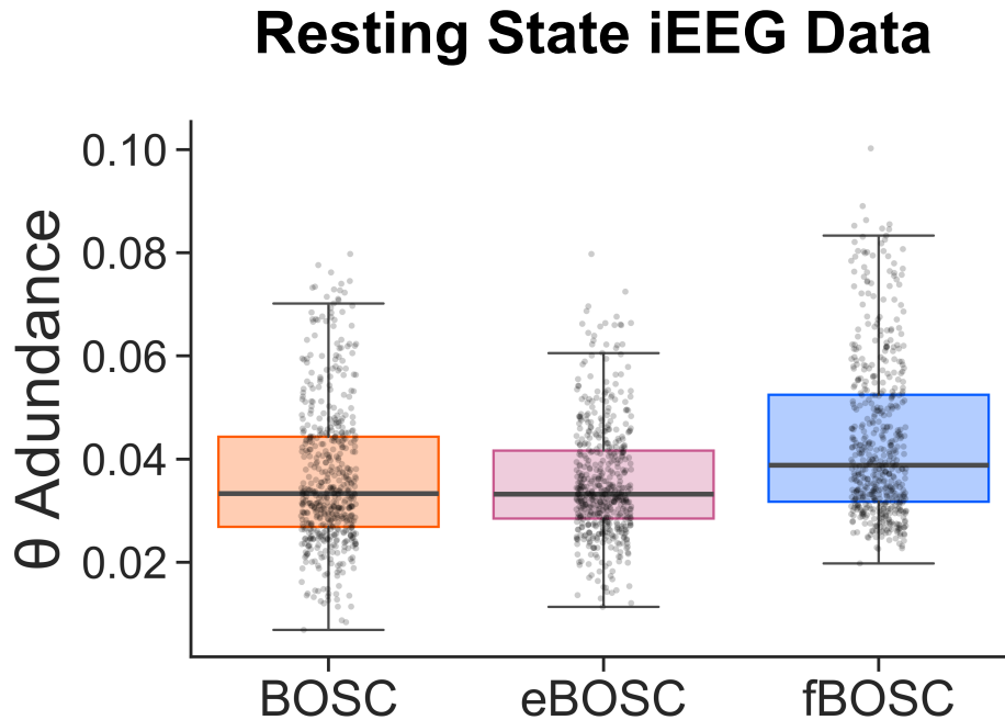
FIGURE 7 Using resting state iEEG data from 10 patients, theta (3-7 Hz) burst abundance was quantified as the duration of rhythmic episodes relative to the length of the recording. Abundance values are plotted separately for each method. Individual data points correspond to each of the 533 electrodes across the 10 patients.
