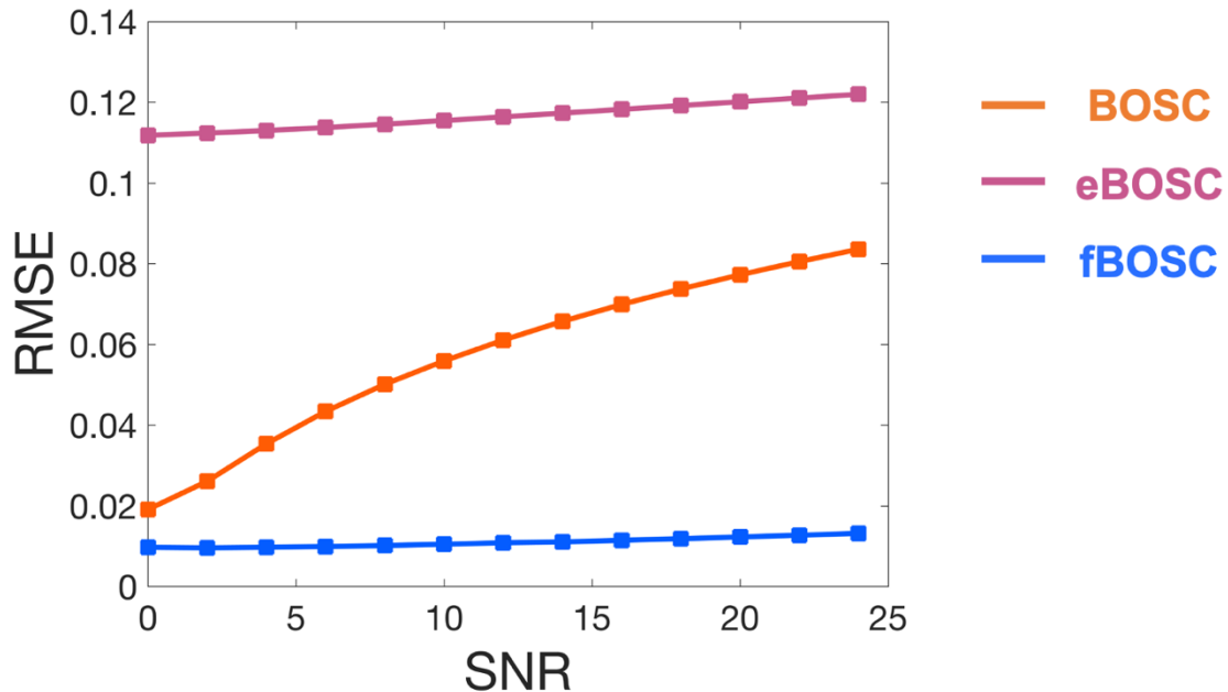
FIGURE 3 Simulations using data with a non-linear 1/f power spectrum and embedded theta and alpha bursts. The signal-to-noise ratio (SNR) of the bursts was increased from 0-24, in steps of 2. The root mean squared error (RMSE) between the estimated and actual 1/f fit was plotted for BOSC, eBOSC and fBOSC for each of the SNRs.
