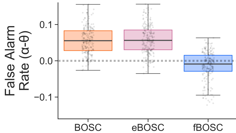
SUPPORTING FIGURE S2 Simulations were performed using data with a non-linear 1/f power spectrum and embedded theta or alpha bursts (SNR = 24). BOSC, eBOSC and fBOSC were used to detect these oscillatory bursts. The difference in false-alarm rate between theta and alpha burst detection is plotted, with an additional dotted line at 0. Across all plots, individual data points correspond to each simulated trial. Note that fBOSC is much closer to 0 than the other two methods, indicating smaller differences in the false alarm rate between frequency bands. Hit-rate is not plotted because the high SNR bursts caused ceiling effects, i.e. the hit-rate was nearly always equal to 1 for each trial.
