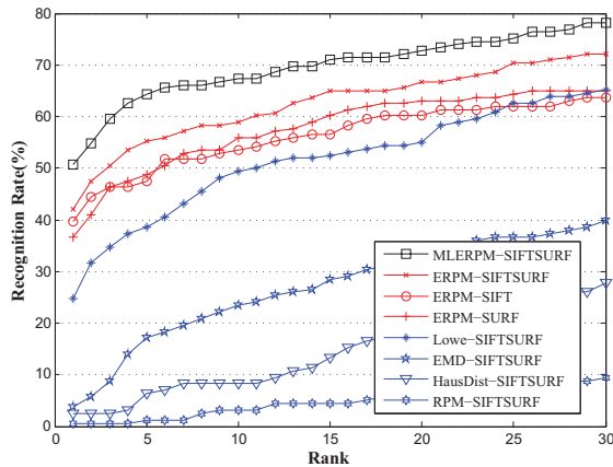
Figure 8. Recognition rates of the comparing algorithms at various ranks on LFW
