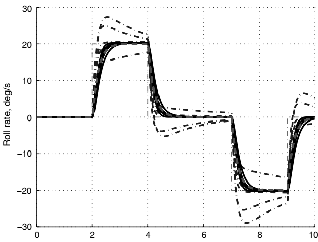
a) Roll rate, deg/s b) Pitch rate, deg/s Fig. 4 The inner loop response of the UAV controlled using NDI, INDI, and PINDI, subject to mismatches in the aerodynamic model, both in stability and control derivatives. The NDI and PINDI controllers are subject to sensor measurement time delays, and the INDI controlled system is not.
