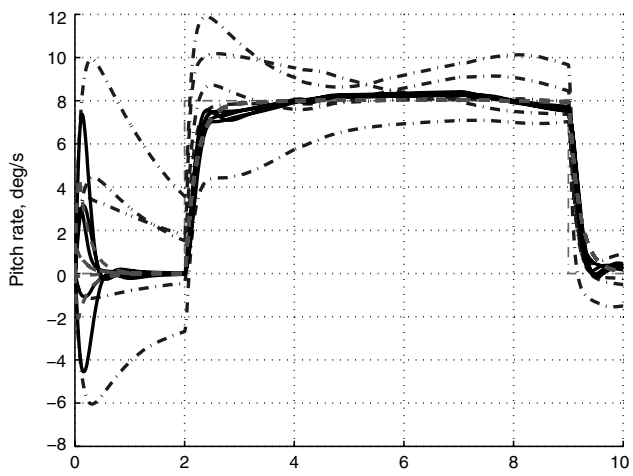
a) Roll rate, deg/s b) Pitch rate, deg/s Fig. 4 The inner loop response of the UAV controlled using NDI, INDI, and PINDI, subject to mismatches in the aerodynamic model, both in stability and control derivatives. The NDI and PINDI controllers are subject to sensor measurement time delays, and the INDI controlled system is not.
