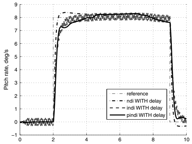
a) Roll rate b) Pitch rate Fig. 3 The inner loop nominal response of the UAV controlled using NDI, INDI, and PINDI. All three control systems are subject to sensor measurement time delays of 10 ms.
