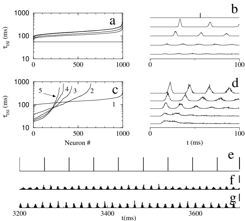
Figure 12. Synchronized network oscillations can exist despite large variations in the individual spiking rates. We plot in (a), (c) the interspike intervals (ISI) of the network neurons sorted from the lowest to highest value, and (b), (d) the ISIHs. In (a), (c) we used different values of the noise strength, from top to bottom D = 0.0, 0.04, 0.08, 0.36, and 0.56 , with \sigma_I = 0 . In (c), (d) from top to bottom \sigma_I = 0 (1), 0.173 (2), 0.346 (3), 0.520 (4), and 0.693 (5), with D = 0.2 . After a transient of 500 ms, the time average is computed over 2 s. We plot the instantaneous firing rate as a function of time for (e) D = 0, \sigma_I = 0 , (f) D = 0.56, \sigma_I = 0 , and (g) D = 0.2, \sigma_I = 0.35 . The scale bars are (e) 500 \text{ imp s}^{-1} , (f), (g) 50 \text{ imp s}^{-1} . We used I = 3.5, \tau_{\text{syn}} = 20, N = 1000, and g_{\text{syn}} = 2.0 .
