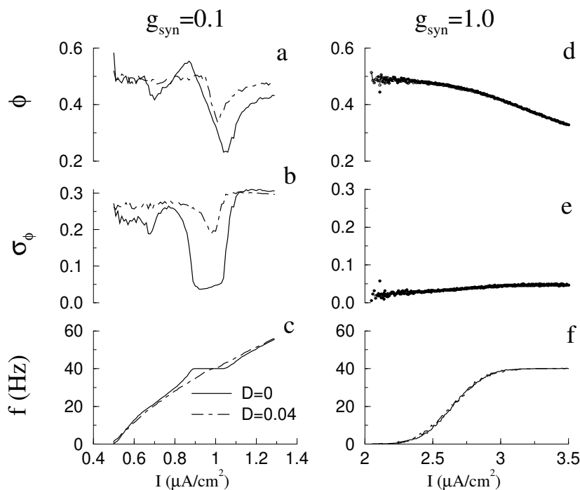
Figure 14. Response of single neuron to simulated network input. We plot in (a), (d) the average phase \phi , (b), (e) the phase jitter \sigma_\phi , and (c), (f) the firing rate f . The coupling strength in (a)–(c) is g_{\text{syn}} = 0.1 , and in (d)–(f) 1.0. The noise strengths are D = 0 (solid curves), and D = 0.04 (dot-dashed curves). In (d), (e) the lines represent running averages over five points, the actual data are denoted by dots. The network input consists of N = 100 neurons of which N_c = 62.5 fire each cycle, \tau_n = 25 , \sigma_c = 0.5 (i.e. CV_W = 0.02 ), and the unitary conductance is g_{\text{syn}}/100 (see the methods section for details). The input phase is defined as \phi = \frac{1}{2} . A transient of 500 ms was discarded, and averages were calculated over 5 \times 10^4 ms.
