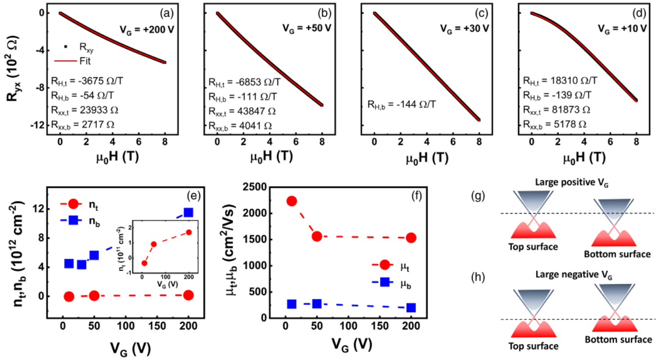
FIG. 2. (a)–(d) Two-band fittings of the Hall resistivity at V_G = +200, +50, +30, and +10 V, respectively. R_{H,t}, R_{H,b} and R_{xx,t}, R_{xx,b} denote the Hall coefficients and sheet resistances for the top and bottom SSs. At V_G = +30 V, the R_{yx} curve is essentially linear, which precludes a meaningful two-band fitting. The resultant Hall coefficient from a linear fit is assigned to R_{H,b} of the bottom surface, which dominates in this transport regime. (e), (f) Carrier densities, n_t and n_b , and the corresponding mobilities \mu_t and \mu_b for the top and bottom SS at each V_G , respectively. Inset: Close-up view of n_t at each V_G . (g), (h) Schematic band structures for the top and bottom SS at large positive and negative V_G 's, respectively.
