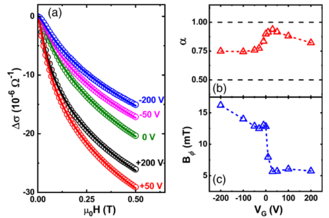
FIG. 3. (a) Magnetoconductivity for the same sample at selected gate voltages at T = 500 mK. Magnetoresistance at higher magnetic fields is shown in Supplemental Material, S4 [49], which includes Refs. [54,55]. The solid lines are fits to the HLN equation. Further details and remarks regarding the fitting can be found in the Supplemental Material, S5 [49]. (b), (c) Best-fit values of \alpha and B_\phi from fittings to the HLN equation at each V_G .
