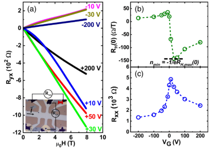
FIG. 1. Ambipolar field effect measured on a 15 nm thick (\text{Bi}_{0.5}\text{Sb}_{0.5})_2\text{Te}_3 epitaxial film on \text{SrTiO}_3 (111). The measurement temperature T = 500 mK. (a) Hall resistivity curves at selected V_G 's. Inset: Optical image of the patterned TI device. The red scale bar measures 300 \mu\text{m} . (b) Zero-field Hall coefficient R_H(0) and (c) corresponding sheet resistance R_{xx} , with varying V_G .
