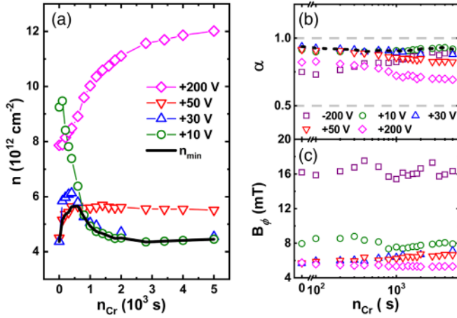
FIG. 4. (a) Electron densities at selected V_G 's with increasing Cr density for the same sample. V_G = +10, +30 , and +50 \text{ V} are close to the surface transport regime. V_G = +200 \text{ V} serves as a reference showing the effect of electron doping by the Cr impurities. The black solid line marks the minimum electron density ( n_{\text{min}} ) identified at each n_{\text{Cr}} . (b) \alpha and (c) B_\phi from fittings of the MC data to the HLN equation at selected V_G 's as functions of Cr density.
