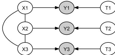
FIG. 2. Graph representing the process generating a t^* -random vector Y from a latent Gaussian random vector X and independent latent Gamma-divisors.
