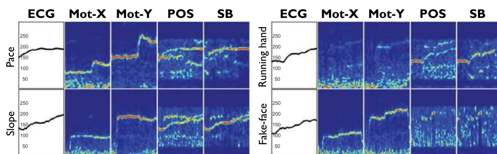
Figure 6. The ECG reference signal and the spectrograms of the horizontal motion (motion-x, denoted as ‘Mot-X’), vertical motion (motion-y, denoted as ‘Mot-Y’), and pulse-signals of POS and SB obtained from the ‘miscellaneous’ category. The signals of Mot-X and Mot-Y are measured using the center of gravity of segmented skin-regions across the video.
