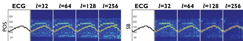
Figure 7. The spectrograms of the pulse-signals of POS and SB obtained on the video of skin-type IV-V (subject 5) using different window lengths. By increasing the window length, the SNR of SB is significantly increased from 0.23 dB to 9.27 dB, whereas the SNR of POS decreases from 1.20 dB to -1.35 dB.
