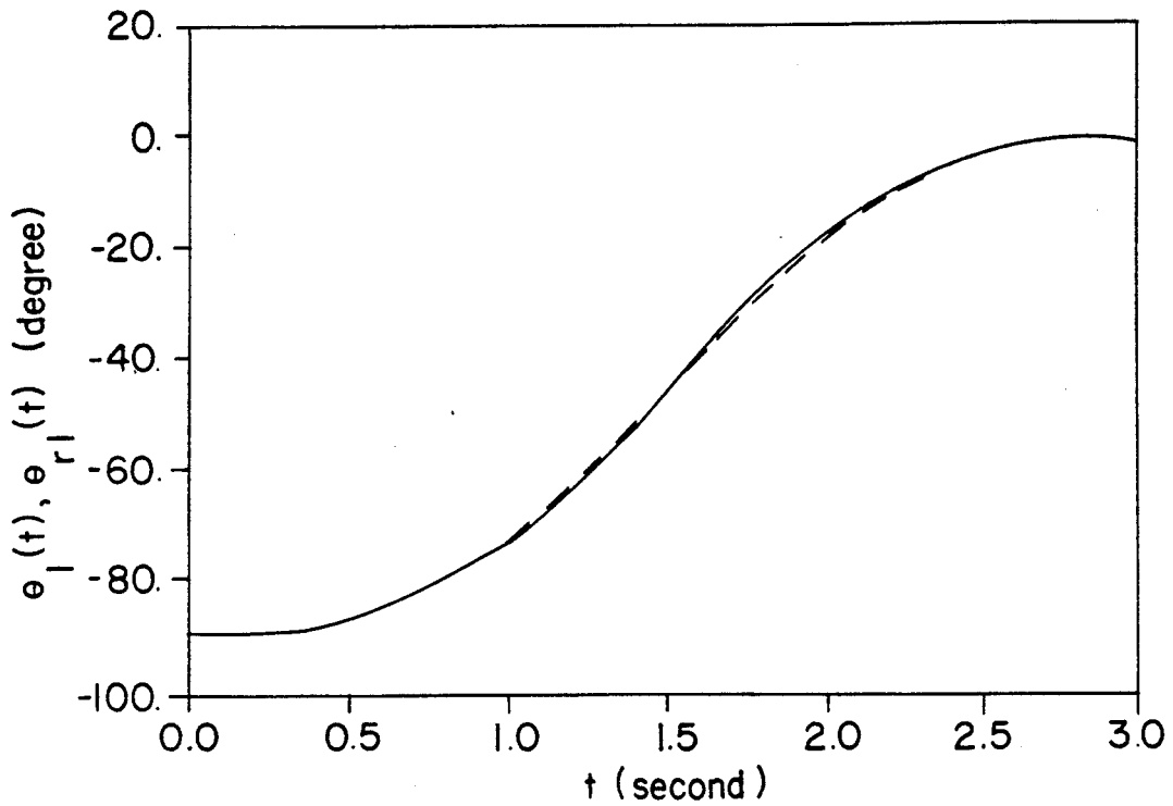
Desired (dashed) and Actual (solid) Trajectories of the Joint Angle e_1(t)
