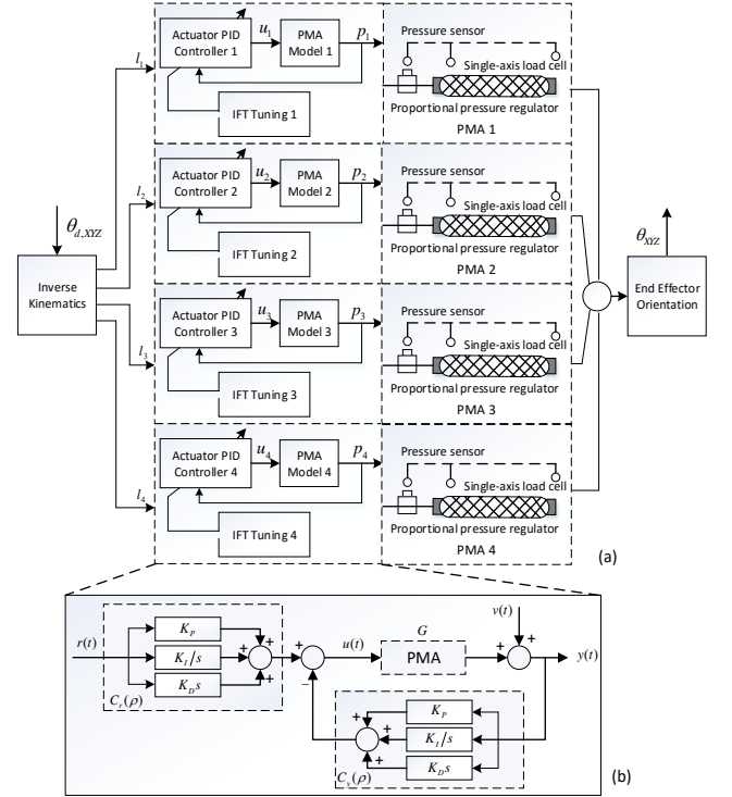
Fig. 3. Control system of the ankle rehabilitation robot. (a) Structure of the multiple DOFs IFT. (b) Diagram of the controller for each PMA.
