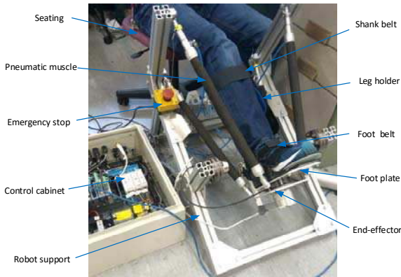
Fig. 5. Configuration of the robot experimental setup with human ankle.
