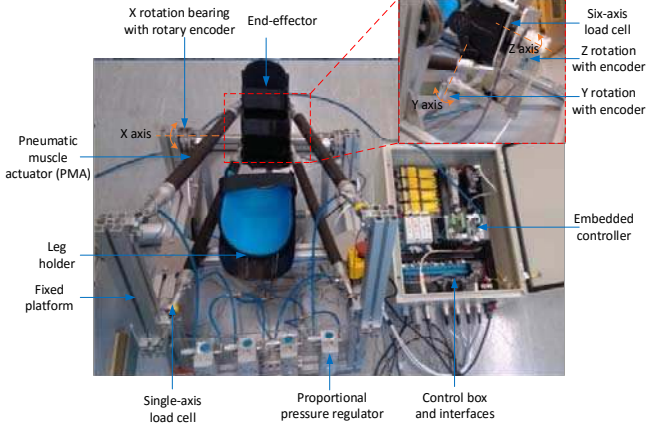
Fig. 1. Prototype of the compliant parallel ankle rehabilitation robot.
