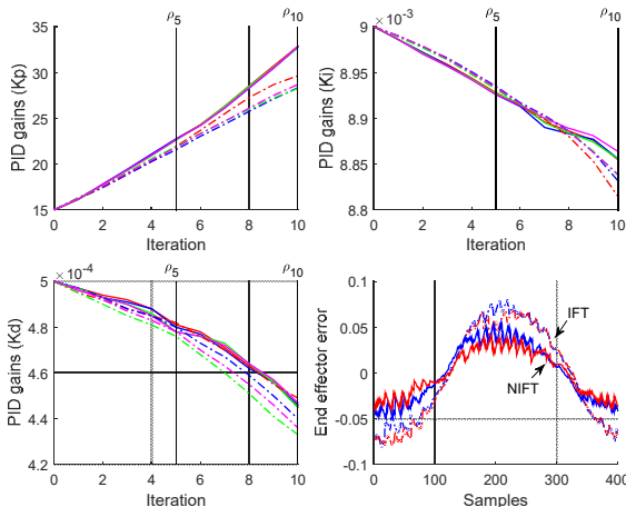
Fig. 8. Robustness test by comparison with standard IFT at \rho_5 and \rho_{10} : solid lines indicate the result of NIFT while dashed lines the IFT; red, blue, green and magenta lines represent the results of actuator 1 to 4, respectively.
