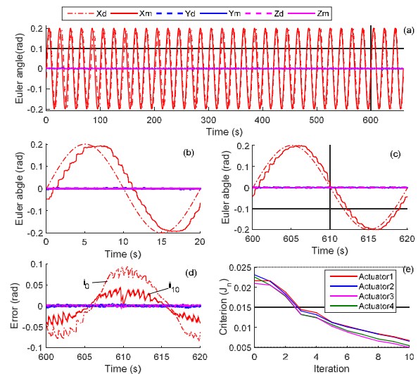
Fig. 4. Repetitive control result using normalised IFT tuning. (a) End-effector orientation during 10 iterations. (b) Tracking result before tuning (iteration 0). (c) After tuning (iteration 10). (d) End-effector errors. (e) Design criteria.
