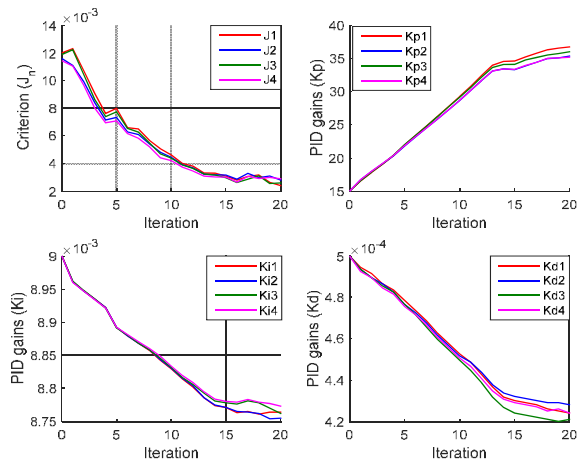
Fig. 10. Convergence test through a case study with 20 iterations: red, blue, green and magenta lines represent the design criteria and PID gains of actuator 1 to 4 of the ankle rehabilitation robot, respectively.
