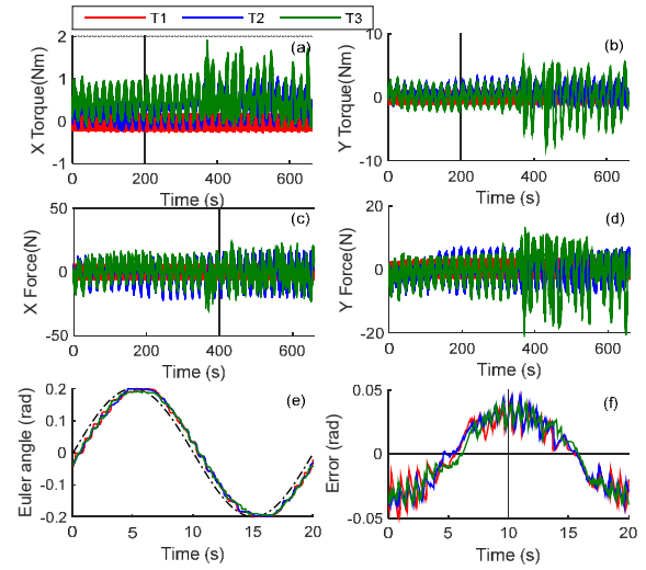
Fig. 6. Experimental results of T1, T2 and T3 with participant 1. (a) Interaction torques about X axis and (b) about Y. (c) Interaction forces along X axis and (d) along Y. (e) End-effector orientation results at the end of tuning. (f) End-effector orientation errors at the end of tuning.
