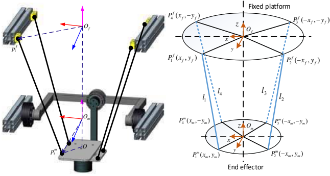
Fig. 2. Kinematic structure of the parallel ankle rehabilitation robot.
