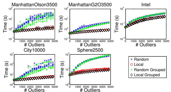
Fig. 4. Scatter plots showing the runtime depending on the number and type of outliers for DCS. DCS does not add significant overheads to the sparse matrix factorization algorithms compared to standard least squares. Local outliers create less fill-in inside and hence requires less time.
