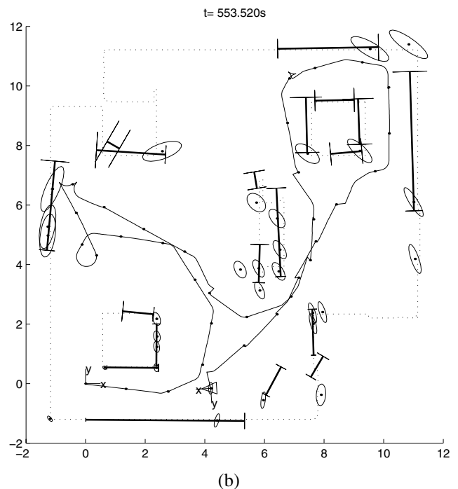
Fig. 8. Global stochastic maps in a loop closing situation. (a) Before loop closing, a local map with features signaled with an arrow has been joined to the global map. (b) The two features have been correctly matched with the corner and the lower wall, and the global map has been updated.
