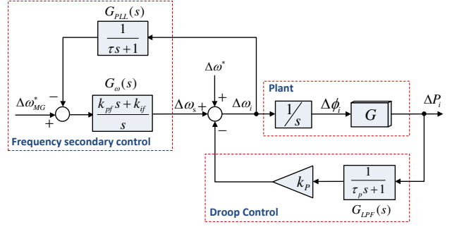
(a) frequency control model
