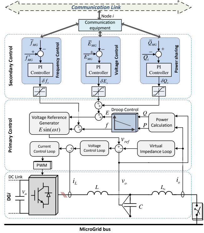
Fig. 3. Details of the proposed DSC for an individual DG in an islanded MG.
