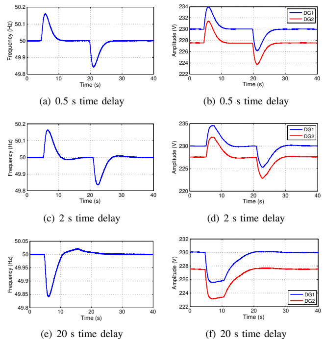
Fig. 17. Experimental evaluation of the proposed DSC in regulating frequency and voltage of the MG considering packet delay.
