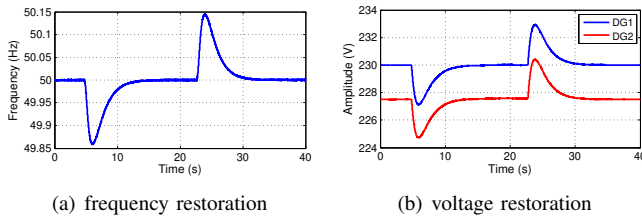
Fig. 18. Evaluation of proposed DSC in regulating frequency and voltage of the MG considering packet losses.
