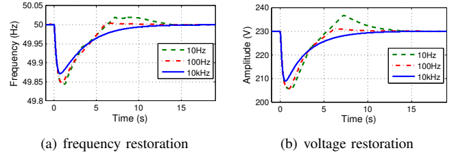
Fig. 13. Impact of packet loss on the performance of proposed DSC considering different sampling rates.
