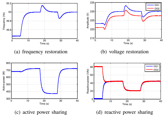
Fig. 16. Experimental validation of proposed algorithm for DSC of an islanded MG with two units.
