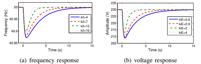
Fig. 11. Verifying sensitivity of the proposed DSC to the PI parameters.
