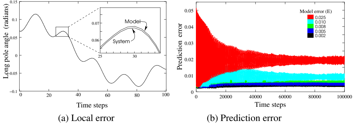
Figure 6.2: Model accuracy (color figure) . Plot (a) shows the trajectory of the long pole angle for the real system (target environment) and model M_{0.002} (simulation environment). A network is controlling the real system and each time step the model is also fed the state and action to produce a one-step prediction. The inset shows that the model is locally very accurate. Plot (b) shows the prediction error for each model. The large errors seen at the beginning of the trial are due to the high velocities of the poles swinging back and forth as the controller gradually stabilizes the system. When velocities are high successive states are further apart and prediction errors are more likely. Models with more error E have greater error in practice.
