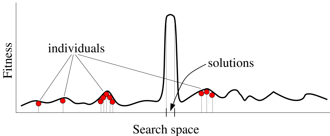
Figure 5.1: A difficult fitness landscape . The curve represents the fitness value of each point in a hypothetical 1-dimensional search space. The red circles are the individual members of the population. Because the solutions represent only a small part of the search space and the fitness landscape is rugged, the initial population may not sample the fitness near this region. As a result the population converges prematurely to a local maxima.
