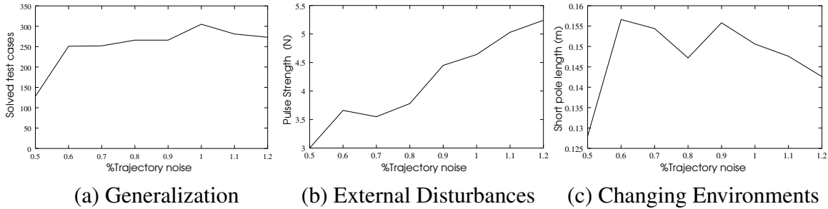
Figure 6.6: Robustness results. The plots show the performance of successfully transferred controllers evolved at different levels of trajectory noise on the three different tests for robustness. Plot (a) shows the number of generalization test cases, on average, solved by the controllers. In plot (b), the y -axis is the average force in Newtons that a network could withstand. In plot (c), the y -axis is the average short pole length that could be balanced for 10,000 time steps. High levels of trajectory noise generally yield more robust behavior in transferred controllers.
