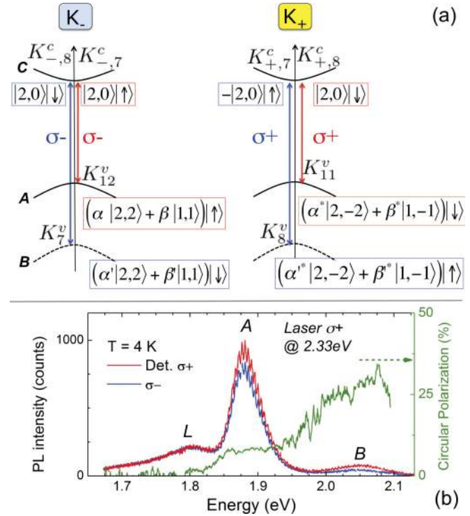
FIG. 2. (Color online) (a) Selection rules for optical dipole transitions in a simple single particle picture in K_+ and K_- valleys at zero magnetic field, adapted from Refs. 8–10; states are represented as |L, M\rangle for valence states, and |\uparrow\rangle ( |\downarrow\rangle ) stand for electron spin up (down). For simplicity, the k -linear term in the CB is neglected, and the A(B) VBs for K_+ and K_- are degenerate in energy. Local trigonal symmetry of electron states at K_{\pm} points is C_{3h} in Koster notation (Ref. 24), with states labeled using corresponding group representations (b). PL spectra at T = 4 K copolarized (red/light gray) and cross polarized (blue/dark gray) with respect to the \sigma^+ polarized highly nonresonant excitation laser at 2.33 eV. Transitions L and A are visible in addition to the B exciton. The small periodic signal variations are due to optical interference in the setup. The (green) right axis shows the PL circular polarization.
